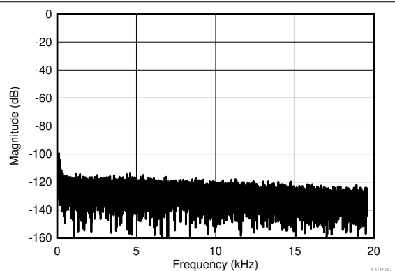
Figure 6-33. Frequency Spectrum With 35Hz Input Signal
