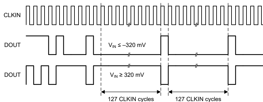
Figure 7-5. Output of the AMC1306M25E in Case of an Input Overage
