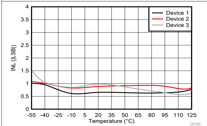
Figure 6-10. Integral Nonlinearity vs Temperature
