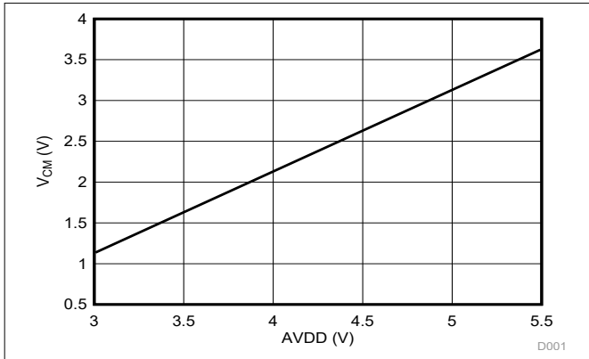
Figure 6-6. Maximum Operating Common-Mode Input Voltage vs High-Side Supply Voltage
