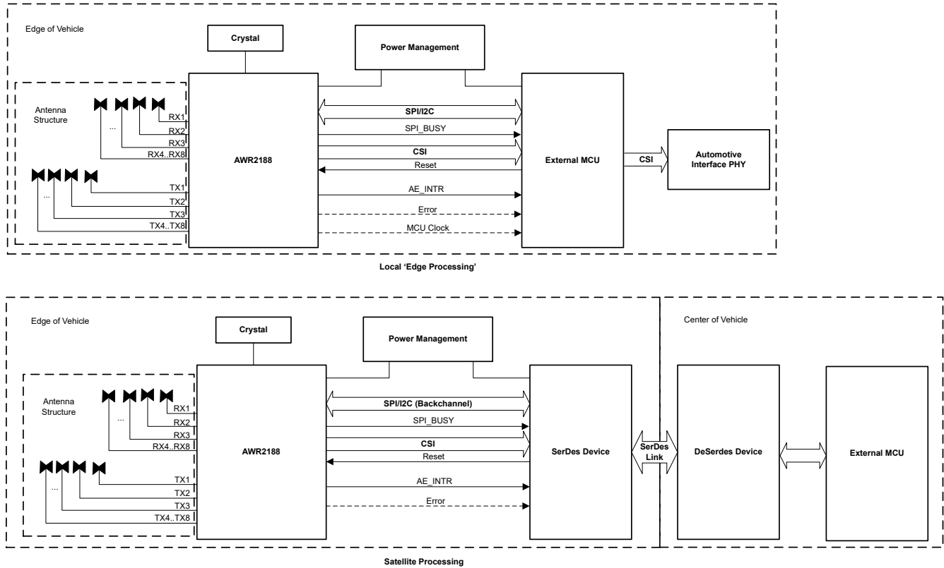
Figure 2-1. Radar Sensor for Automotive Applications
