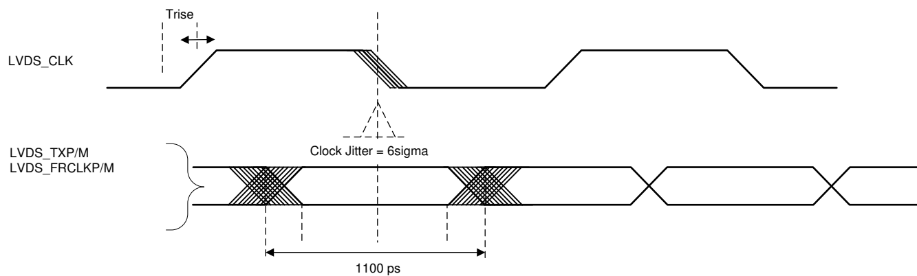
Figure 7-15. Timing Parameters
