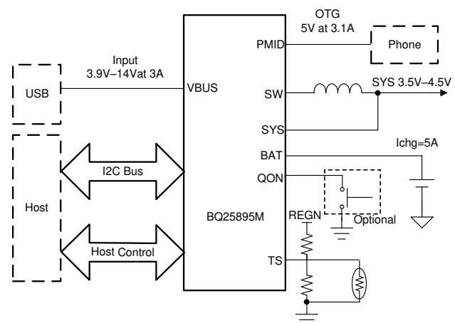
Simplified Schematic
