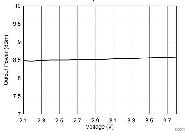
Figure 5-45. TX Bluetooth low energy Maximum Output Power vs VDDSD, 2440 MHz
