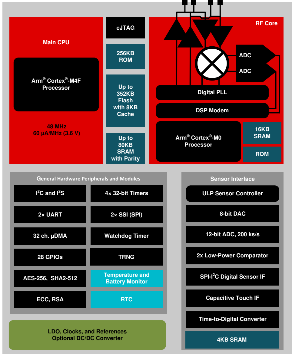
Figure 4-1. CC1352R Block Diagram
