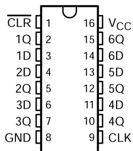
Figure 4-1. CD54ACT174 J Package, 16-PIN CDIP; CD74ACT174 D, N, or PW Package; 16-PIN SOIC, PDIP, or TSSOP (Top View)
