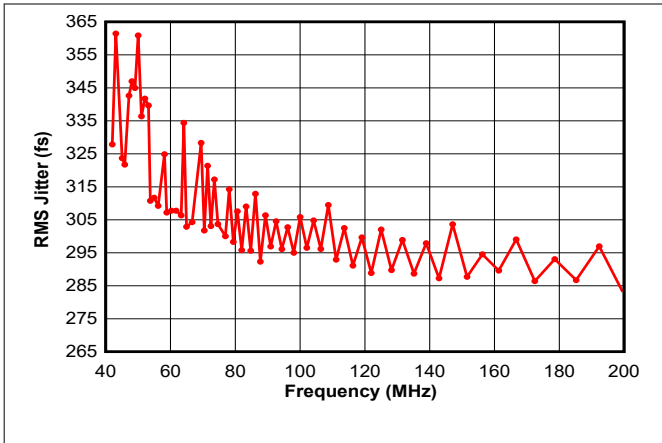
Figure 6-9. Typical RMS Jitter vs Frequency at 3.3V Supply and 25°C (BW 12kHz to 20MHz)
