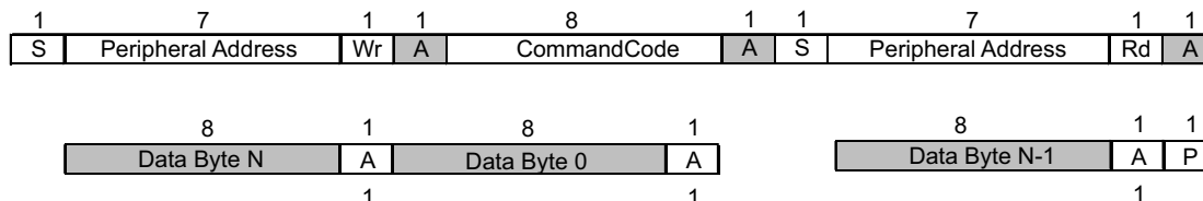
Figure 7-6. Block Read Protocol
