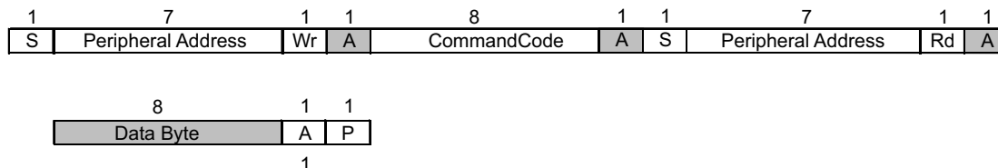
Figure 7-4. Byte Read Protocol
