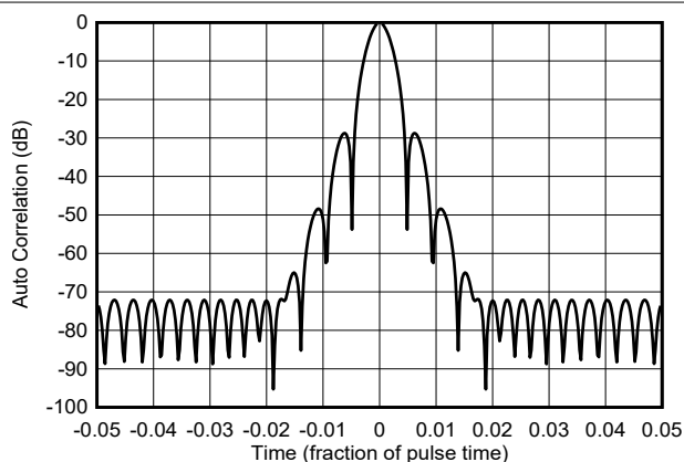
Figure 8-16. Auto-correlation of NLFM Chirp
