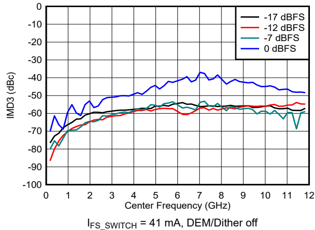
Figure 6-112. IMD3 vs Frequency and Digital Amplitude in NRZ/RF Modes
