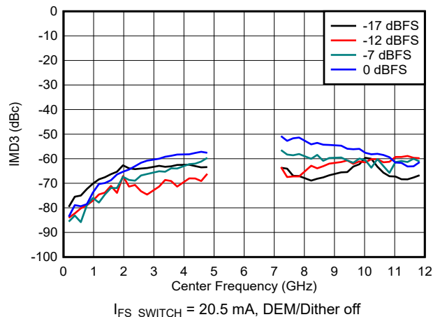
Figure 6-114. IMD3 vs Frequency and Digital Amplitude in DES2X Modes
