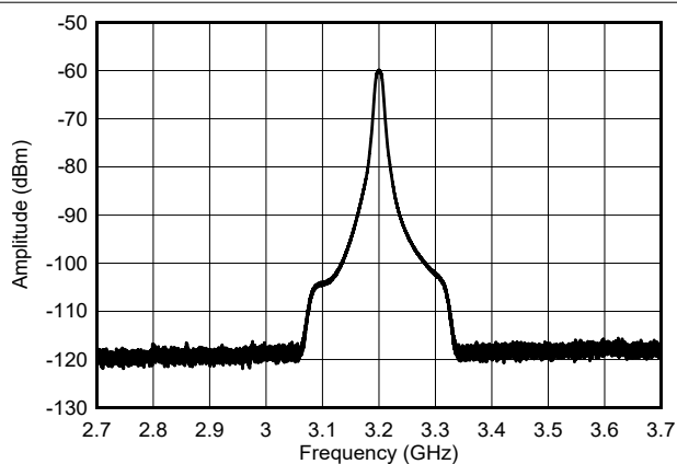
Figure 8-18. NLFM Chirp Output Spectra across 1 GHz
