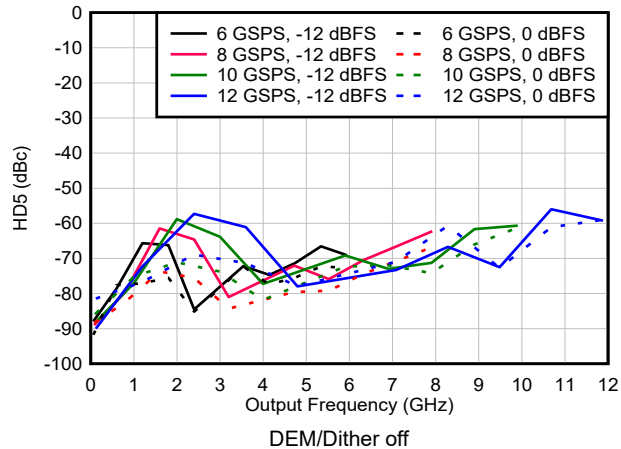
Figure 6-185. HD5 vs Frequency and Sample Rate in DES2X Modes
