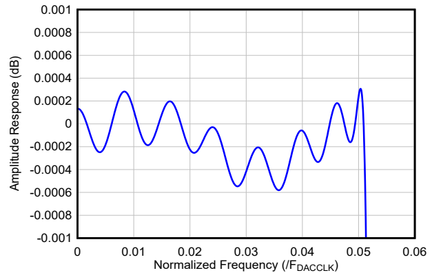
Figure 7-16. 8x Interpolation Filter Passband Response
