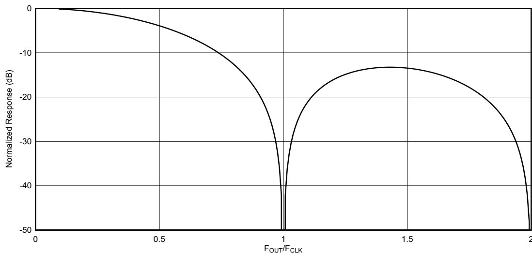
Figure 7-2. NRZ Mode Output Frequency Response
