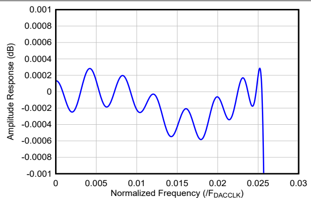
Figure 7-20. 16x Interpolation Filter Passband Response
