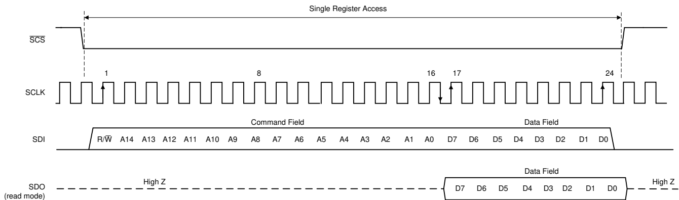
Figure 8-1. Serial Interface Protocol: Single Read and Write
