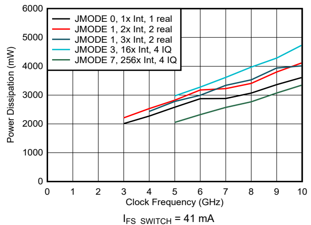
Figure 6-212. Power Dissipation vs Clock Frequency and Digital Mode
