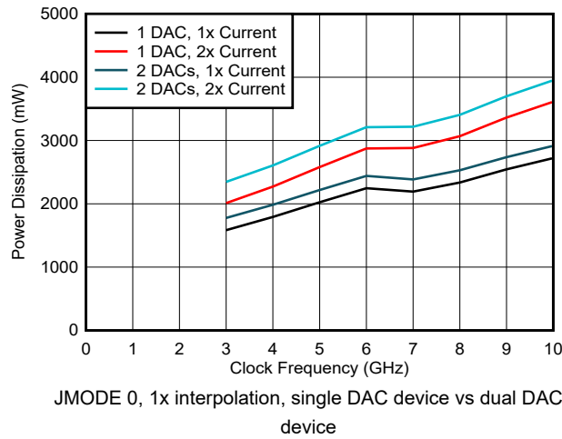
Figure 6-215. Power Dissipation vs Clock Frequency and DAC Mode
