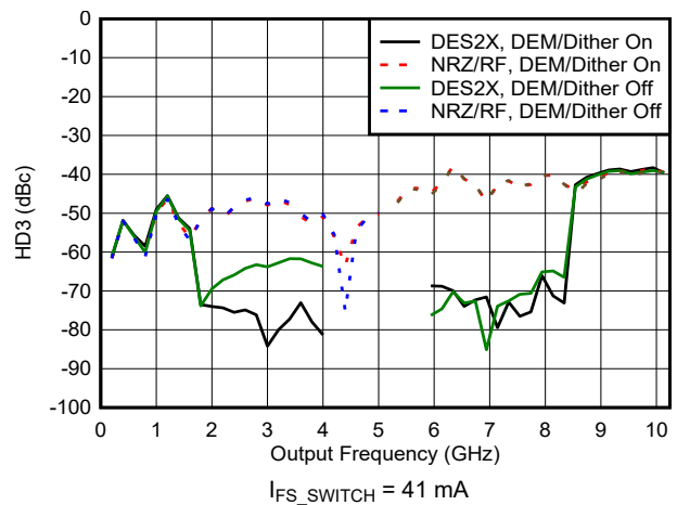
Figure 6-96. HD3 vs Frequency and Mode
