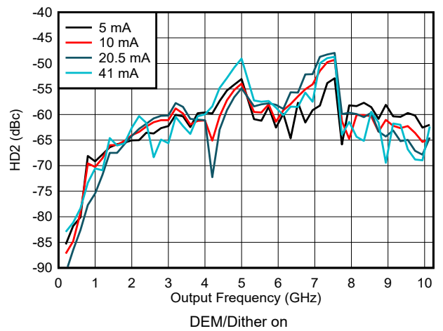
Figure 6-142. HD2 vs Frequency and Output Current in NRZ/RF Modes
