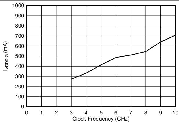
Figure 6-225. VDDDIG Current vs Clock Frequency
