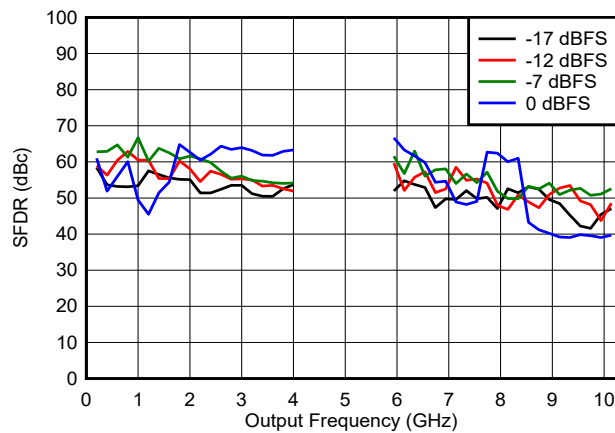
Figure 6-107. SFDR vs Frequency and Digital Amplitude in DES2X Modes
