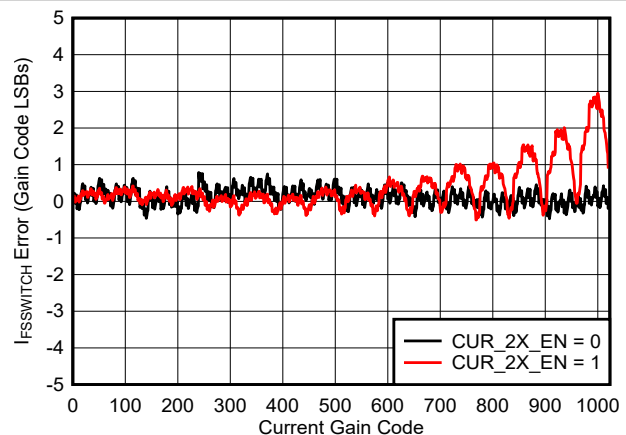
Figure 6-15. I_{\text{FS\_SWITCH}} vs Gain Code
