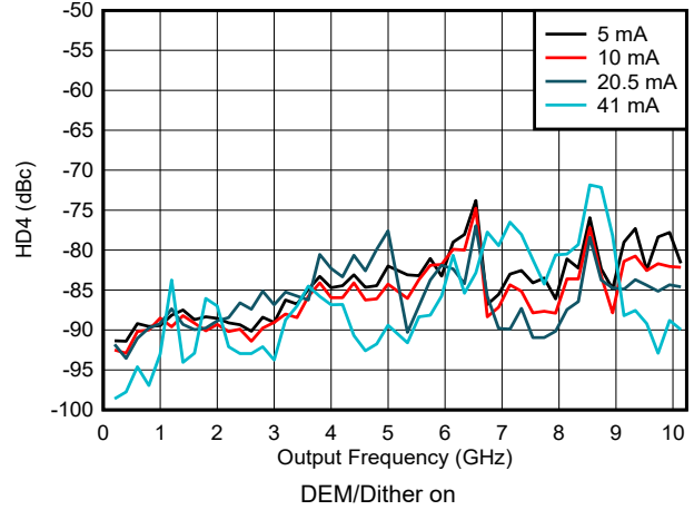
Figure 6-174. HD4 vs Frequency and Output Current in NRZ/RF Modes
