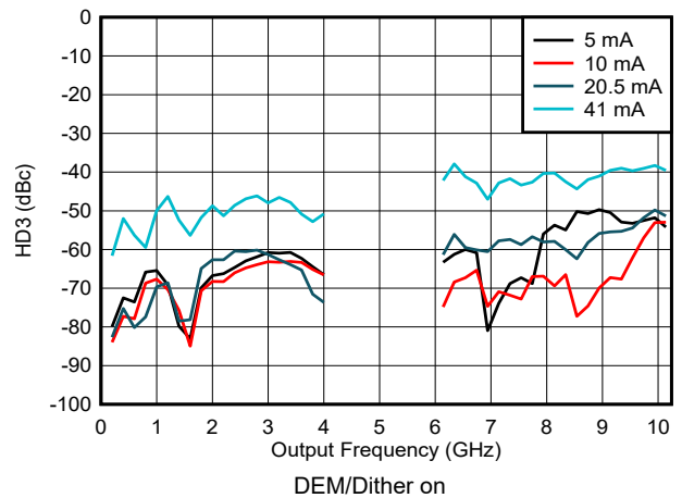
Figure 6-158. HD3 vs Frequency and Output Current in NRZ/RF Modes
