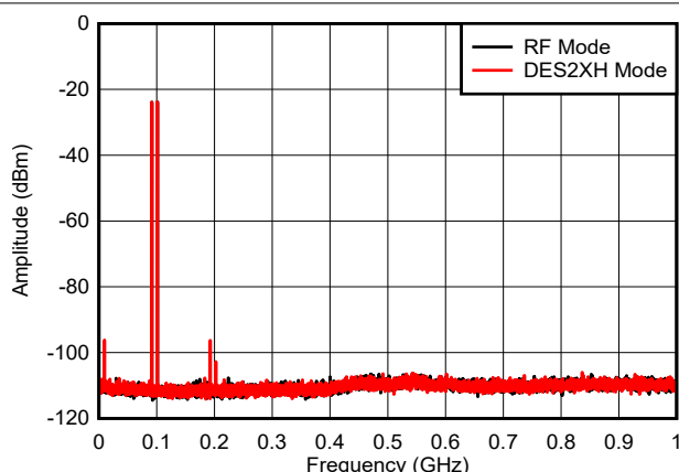
Figure 6-40. Dual Tone, f_{\text{OUT}} = 97\text{ MHz} , -6 dBFS (0 - 1 GHz)
