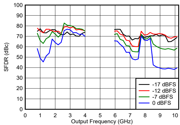
Figure 6-108. SFDR vs Frequency and Digital Amplitude in DES2X Modes
