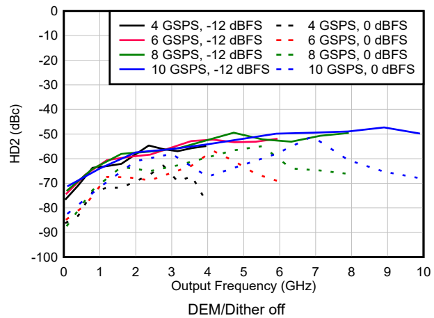
Figure 6-154. HD2 vs Frequency and Sample Rate in NRZ/RF Modes
