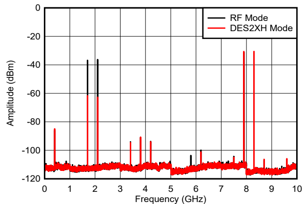
Figure 6-55. Dual Tone, f_{\text{OUT}} = 8097\text{ MHz} , 0 dBFS
