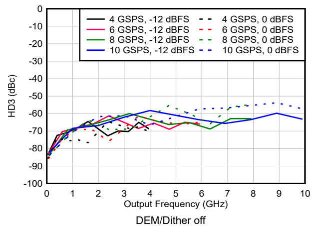
Figure 6-170. HD3 vs Frequency and Sample Rate in NRZ/RF Modes
