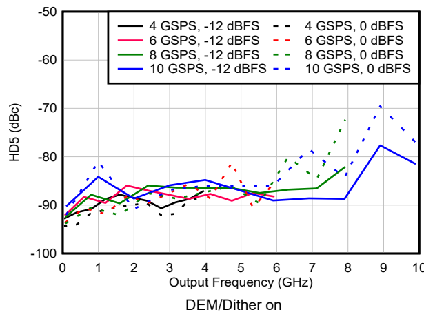
Figure 6-189. HD5 vs Frequency and Sample Rate in NRZ/RF Modes
