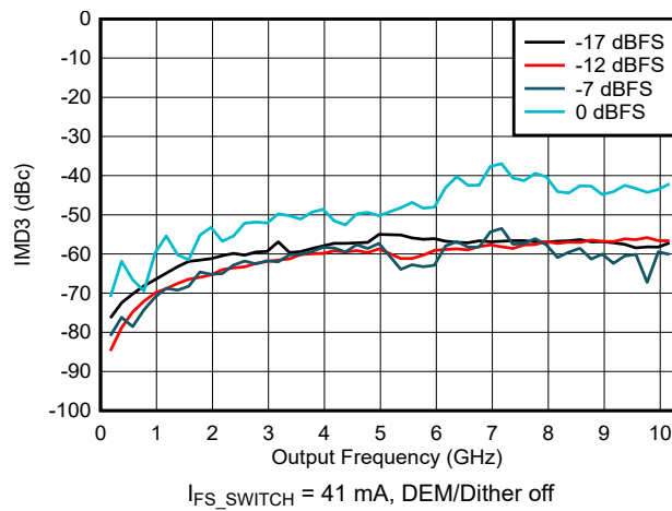
Figure 6-119. IMD3 vs Frequency and Digital Amplitude in NRZ/RF Modes
