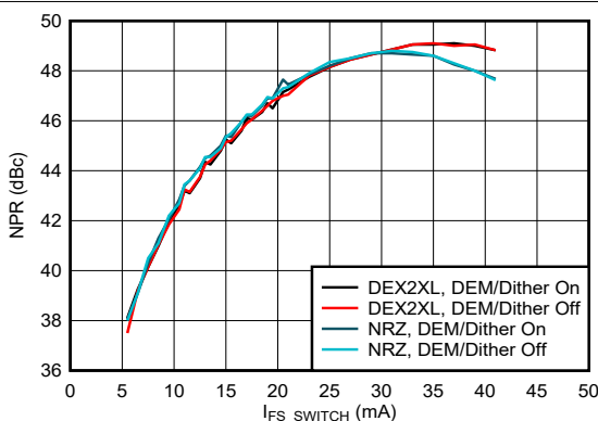
Figure 6-199. Noise Power Ratio vs Output Current: 1 st Nyquist Zone
