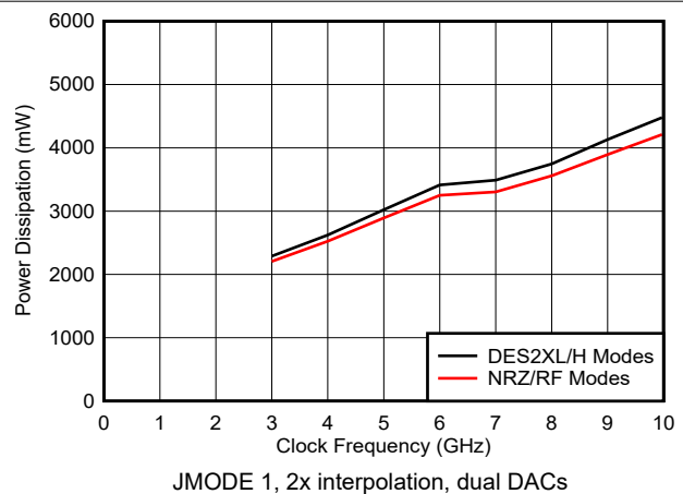
Figure 6-214. Power Dissipation vs Clock Frequency and DAC Mode
