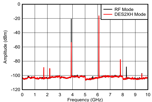
Figure 6-32. f_{\text{OUT}} = 6097\text{ MHz} , -6 dBFS
