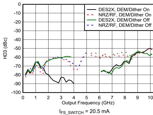
Figure 6-95. HD3 vs Frequency and Mode
