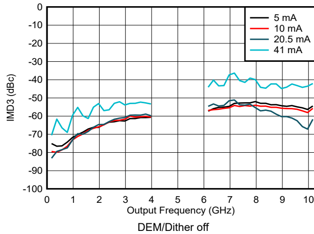
Figure 6-115. IMD3 vs Frequency and Output Current in DES2X Modes
