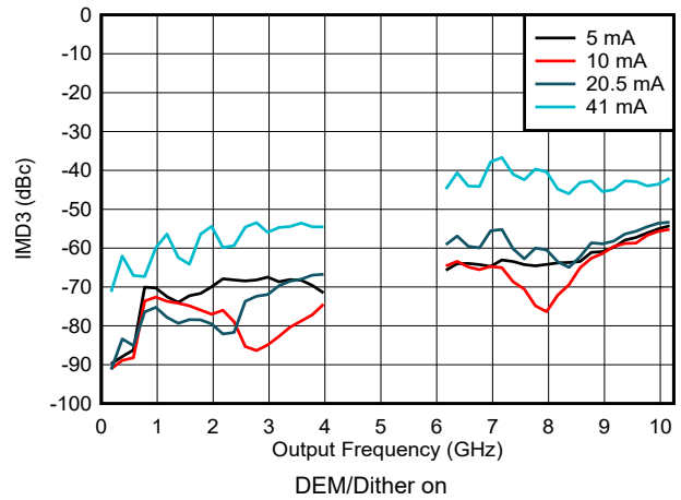
Figure 6-116. IMD3 vs Frequency and Output Current in DES2X Modes
