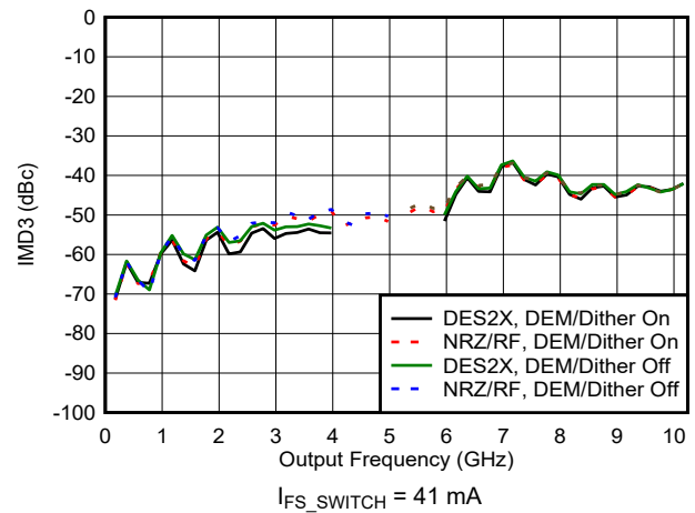
Figure 6-92. IMD3 vs Frequency and Mode
