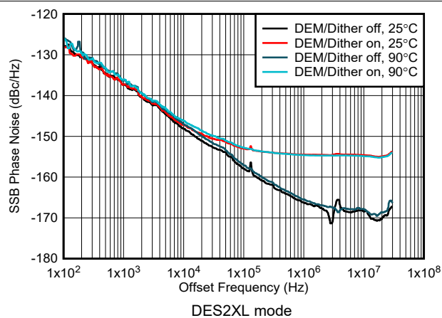
Figure 6-205. Phase Noise vs Offset Frequency at 1 GHz
