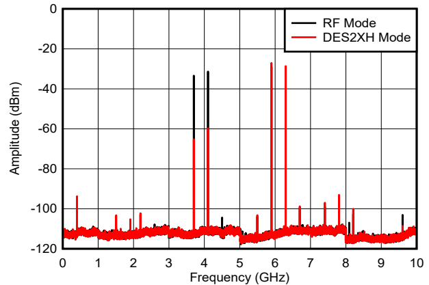
Figure 6-52. Dual Tone, f_{\text{OUT}} = 6097\text{ MHz} , 0 dBFS
