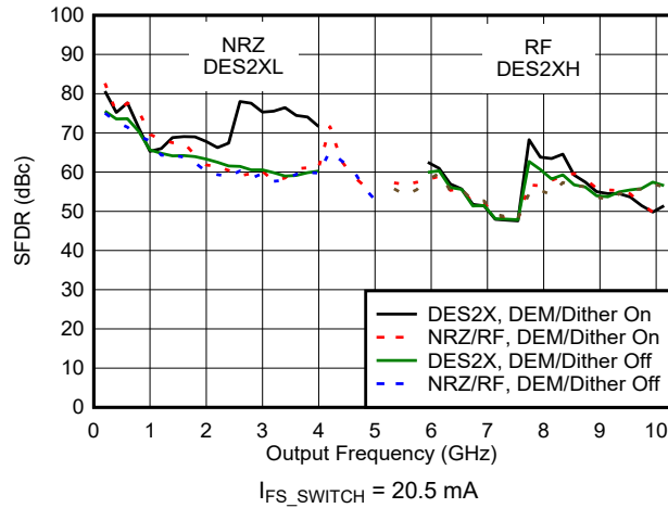
Figure 6-89. SFDR vs Frequency and Mode
