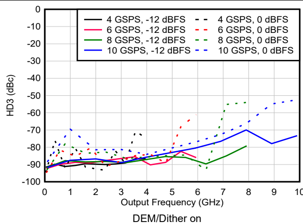
Figure 6-171. HD3 vs Frequency and Sample Rate in DES2X Modes
