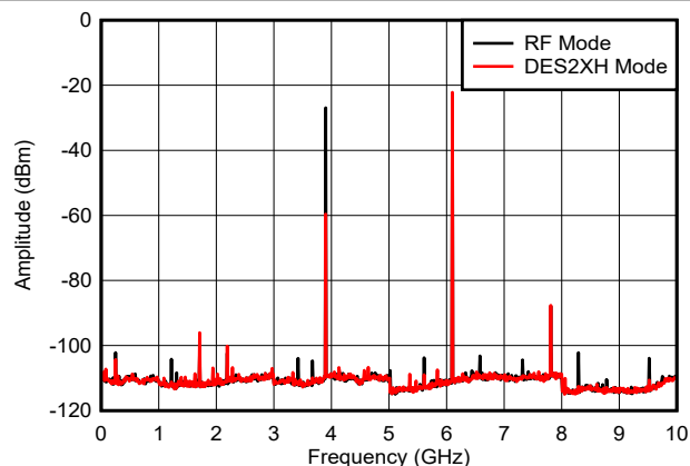
Figure 6-31. f_{\text{OUT}} = 6097\text{ MHz} , 0 dBFS
