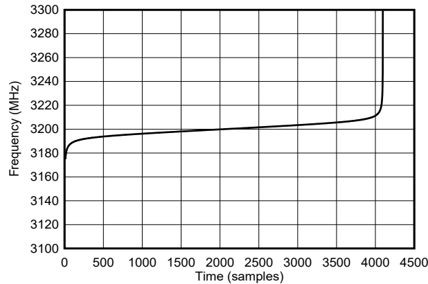
Figure 8-14. NLFM Frequency Ramp
