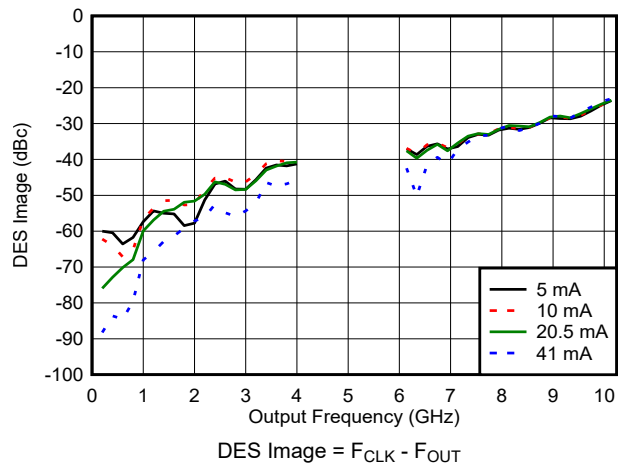
Figure 6-193. DES Image vs Frequency and Output Current in DES2X Modes
