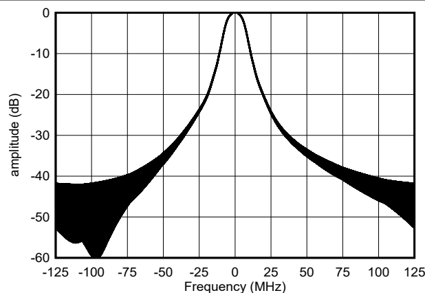
Figure 8-16. Digital Spectrum for NLFM Chirp
