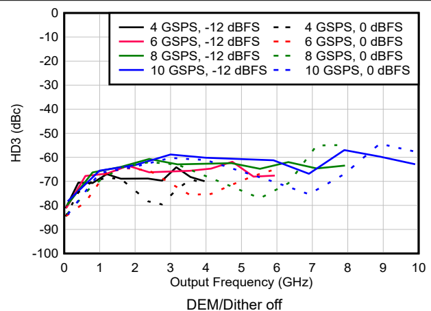
Figure 6-172. HD3 vs Frequency and Sample Rate in DES2X Modes
