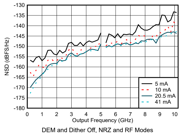
Figure 6-61. NSD vs Output Frequency and Output Current
