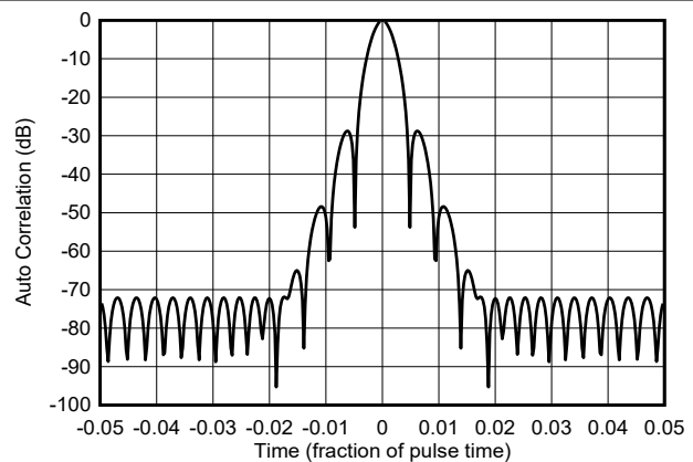
Figure 8-17. Auto-correlation of NLFM Chirp
