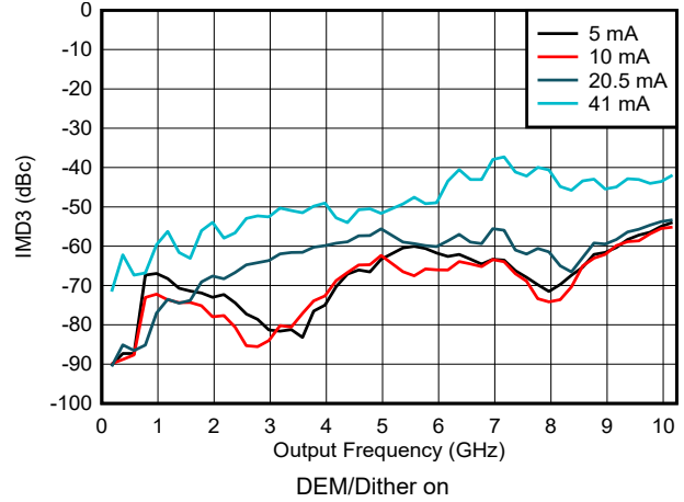
Figure 6-114. IMD3 vs Frequency and Output Current in NRZ/RF Modes
