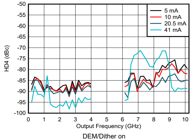
Figure 6-176. HD4 vs Frequency and Output Current in DES2X Modes
