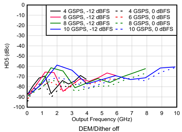
Figure 6-192. HD5 vs Frequency and Sample Rate in DES2X Modes
