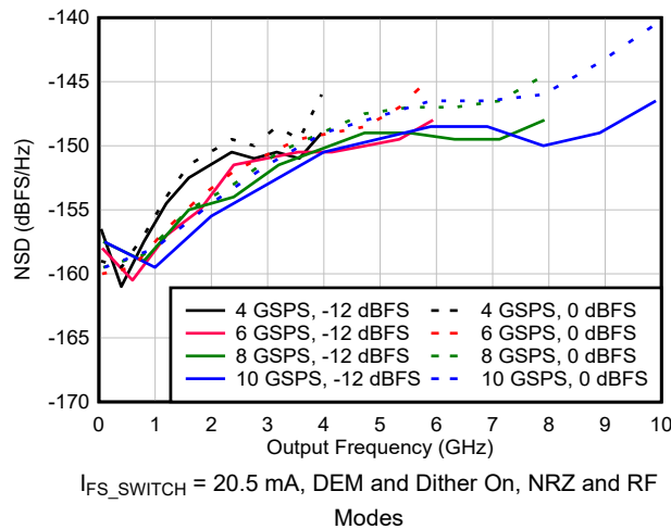
Figure 6-78. NSD vs Output Frequency and Sample Rate
