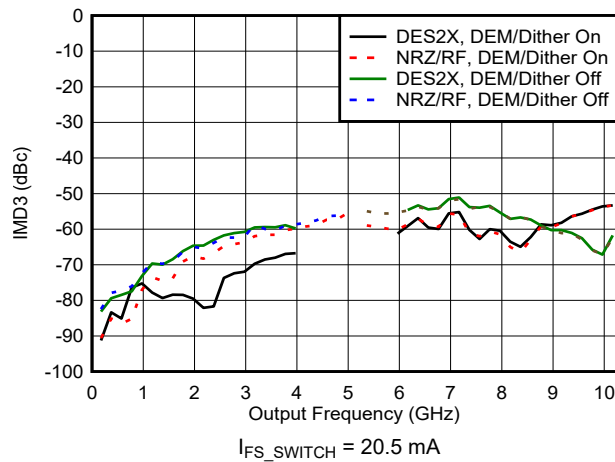
Figure 6-91. IMD3 vs Frequency and Mode
