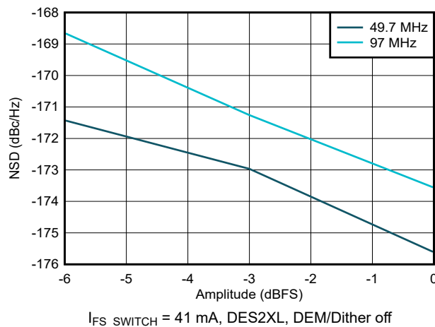
Figure 6-60. NSD vs Digital Amplitude at Low Frequency
