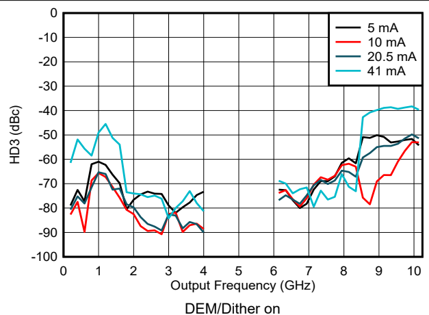
Figure 6-160. HD3 vs Frequency and Output Current in DES2X Modes
