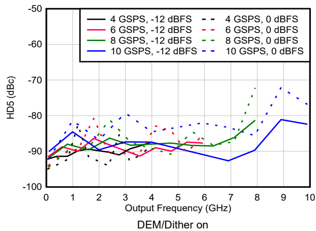
Figure 6-191. HD5 vs Frequency and Sample Rate in DES2X Modes
