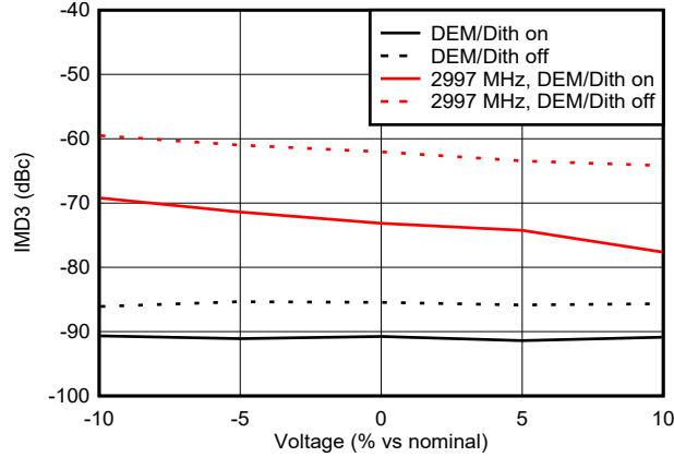
Figure 6-137. IMD3 vs Voltage in NRZ Mode
