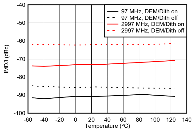
Figure 6-133. IMD3 vs Temperature in NRZ Mode
