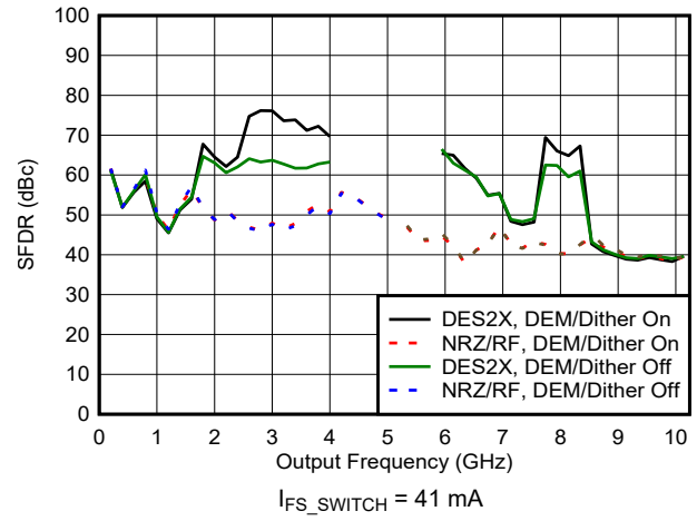
Figure 6-90. SFDR vs Frequency and Mode
