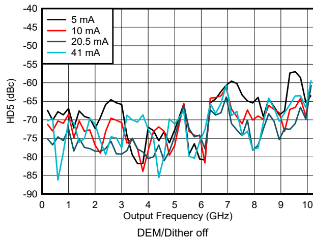
Figure 6-177. HD5 vs Frequency and Output Current in NRZ/RF Modes
