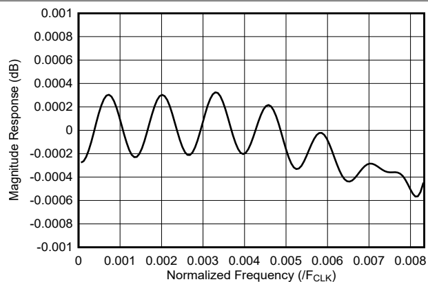
Figure 7-33. 48x Interpolation Filter Passband Response
