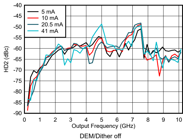
Figure 6-141. HD2 vs Frequency and Output Current in NRZ/RF Modes
