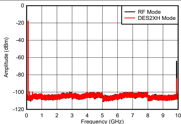
Figure 6-37. Dual Tone, f_{\text{OUT}} = 97\text{ MHz} , 0 dBFS (0 - f_{\text{CLK}} )
