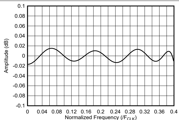
Figure 7-49. DES Interpolator Frequency Response (Passband)
