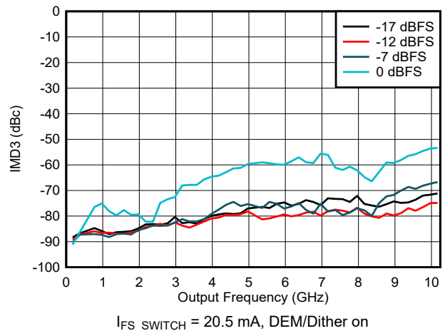
Figure 6-118. IMD3 vs Frequency and Digital Amplitude in NRZ/RF Modes
