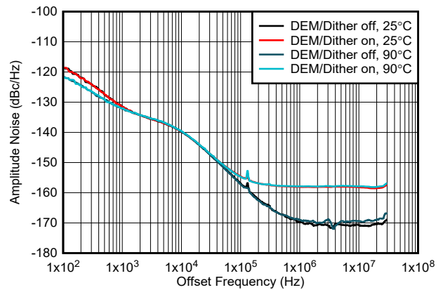
Figure 6-210. Amplitude Noise vs Offset Frequency and Temperature at 1 GHz
