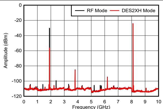
Figure 6-34. f_{\text{OUT}} = 8097\text{ MHz} , 0 dBFS
