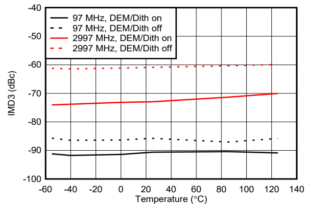
Figure 6-134. IMD3 vs Temperature in DES2XL Mode
