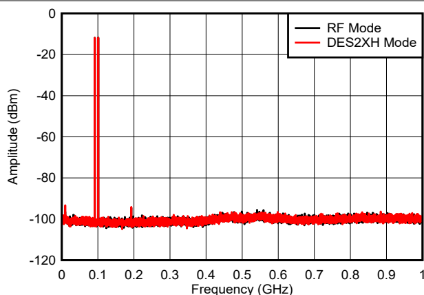
Figure 6-38. Dual Tone, f_{\text{OUT}} = 97\text{ MHz} , 0 dBFS (0 - 1 GHz)
