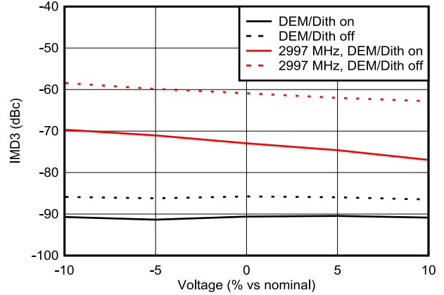
Figure 6-138. IMD3 vs Voltage in DES2XL Mode
