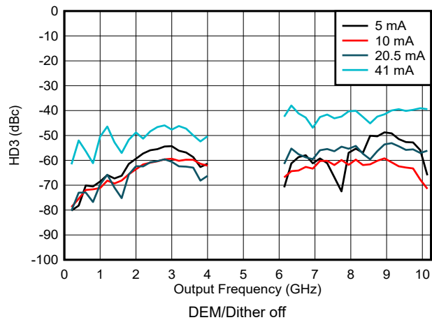
Figure 6-157. HD3 vs Frequency and Output Current in NRZ/RF Modes
