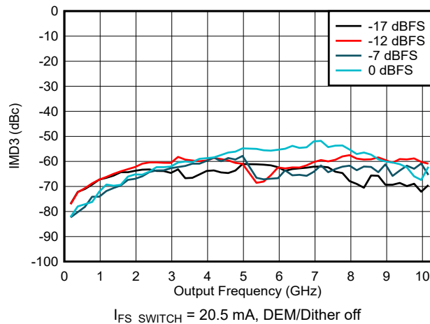
Figure 6-117. IMD3 vs Frequency and Digital Amplitude in NRZ/RF Modes
