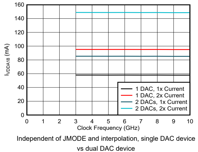
Figure 6-216. VDDA18 Current vs Clock Frequency and DAC Mode
