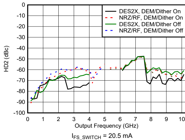
Figure 6-93. HD2 vs Frequency and Mode
