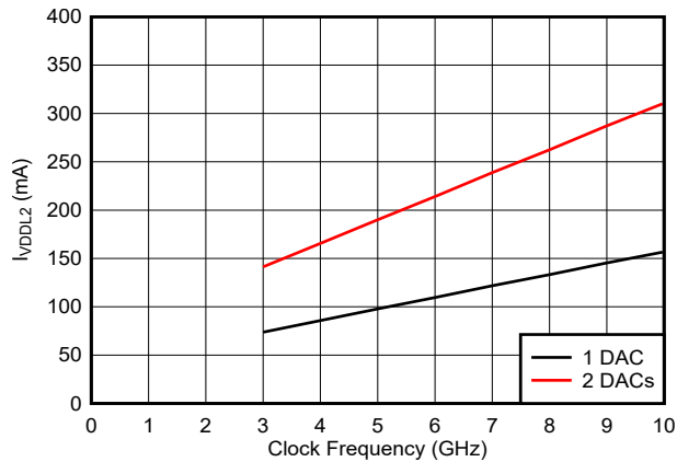
Figure 6-219. VDDLx Current vs Clock Frequency
