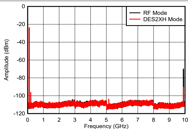
Figure 6-39. Dual Tone, f_{\text{OUT}} = 97\text{ MHz} , -6 dBFS (0 - f_{\text{CLK}} )
