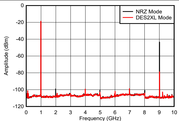
Figure 6-22. f_{\text{OUT}} = 997\text{ MHz} , 0 dBFS
