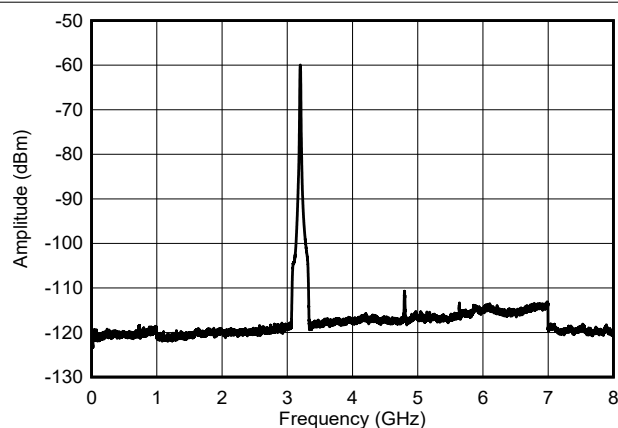
Figure 8-18. NLFM Chirp Output Spectra across 0 - 8 GHz
