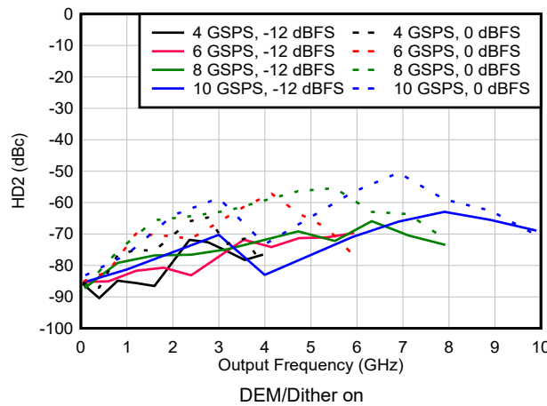
Figure 6-153. HD2 vs Frequency and Sample Rate in NRZ/RF Modes
