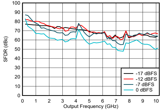
Figure 6-102. SFDR vs Frequency and Digital Amplitude in NRZ/RF Modes
