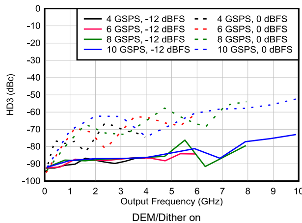
Figure 6-169. HD3 vs Frequency and Sample Rate in NRZ/RF Modes
