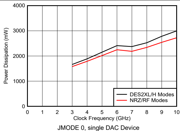
Figure 6-213. Power Dissipation vs Clock Frequency and DAC Mode
