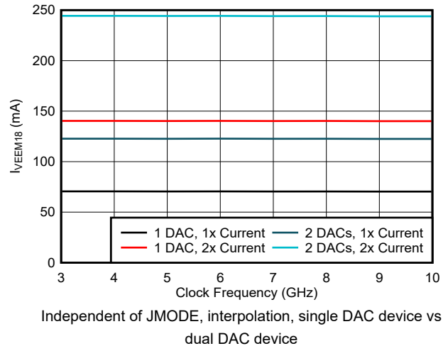
Figure 6-218. VEEM18 Current vs Clock Frequency and DAC Mode
