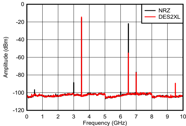
includes PCB, cable and balun loss Figure 6-29. f_{\text{OUT}} = 3497\text{ MHz} , -6 dBFS
