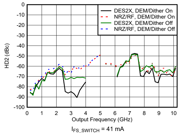
Figure 6-94. HD2 vs Frequency and Mode
