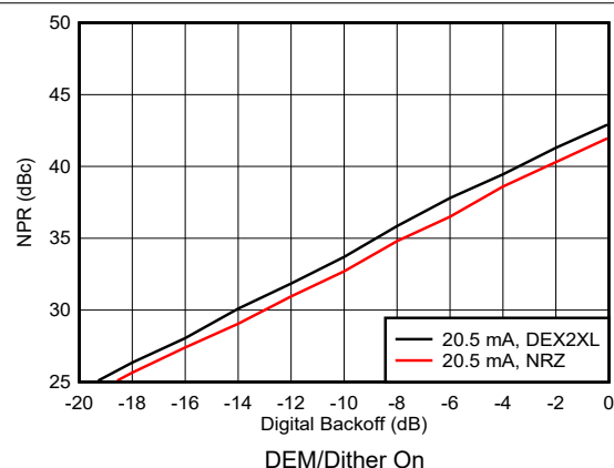
Figure 6-198. Noise Power Ratio vs Digital Backoff: 2 nd Nyquist Zone
