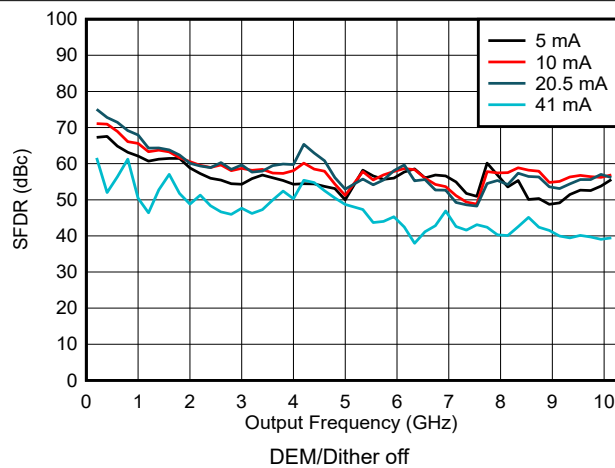
Figure 6-97. SFDR vs Frequency and Output Current in NRZ/RF Modes
