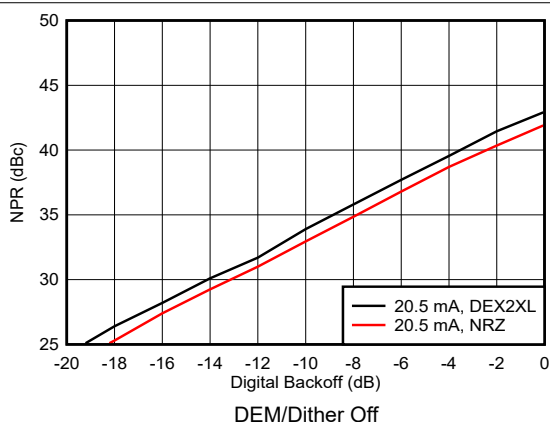
Figure 6-197. Noise Power Ratio vs Digital Backoff: 2 nd Nyquist Zone
