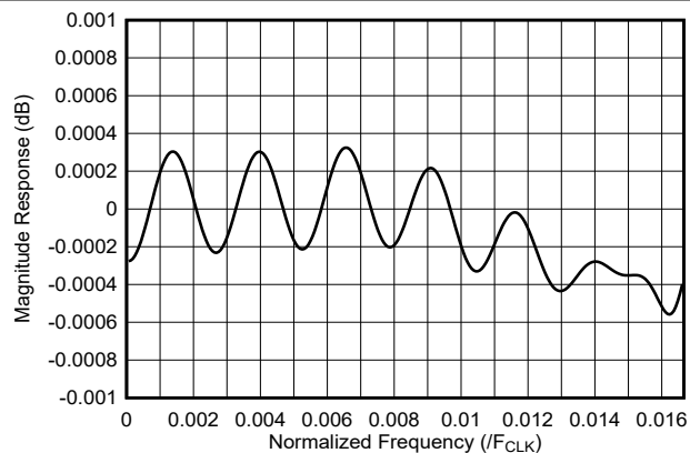
Figure 7-29. 24x Interpolation Filter Passband Response
