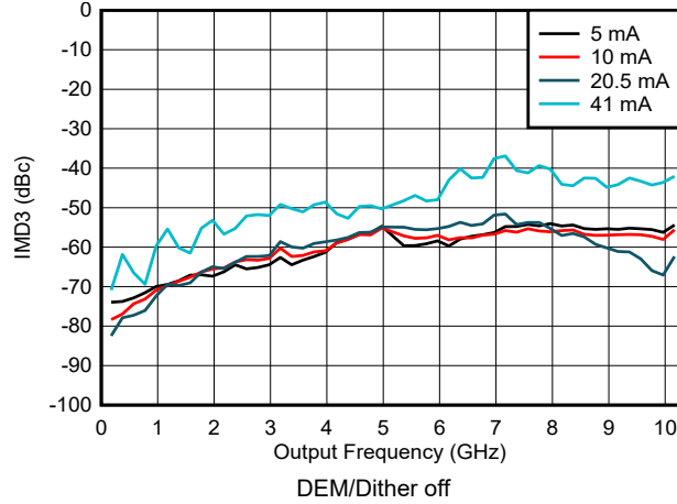
Figure 6-113. IMD3 vs Frequency and Output Current in NRZ/RF Modes
