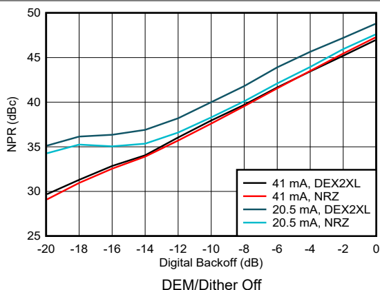
Figure 6-195. Noise Power Ratio vs Digital Backoff: 1 st Nyquist Zone
