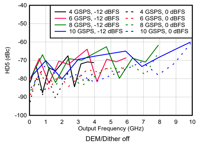
Figure 6-190. HD5 vs Frequency and Sample Rate in NRZ/RF Modes
