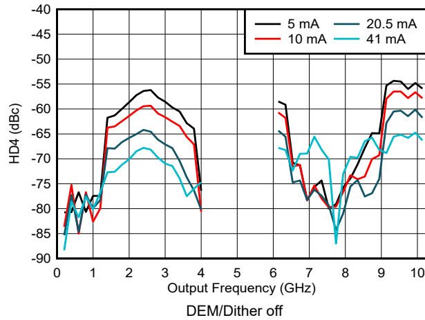
Figure 6-175. HD4 vs Frequency and Output Current in DES2X Modes
