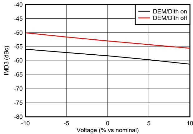
Figure 6-139. IMD3 vs Voltage in RF Mode at 7247 MHz
