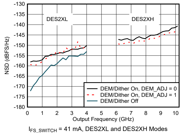
Figure 6-59. NSD vs Output Frequency and DEM/Dither Mode
