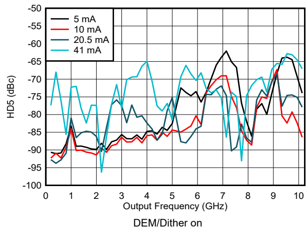
Figure 6-178. HD5 vs Frequency and Output Current in NRZ/RF Modes
