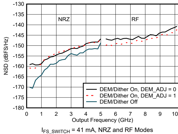
Figure 6-58. NSD vs Output Frequency and DEM/Dither Mode
