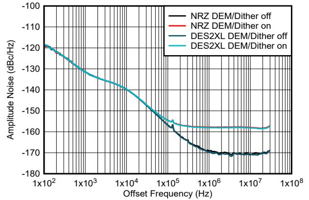
Figure 6-208. Amplitude Noise vs Offset Frequency at 1 GHz
