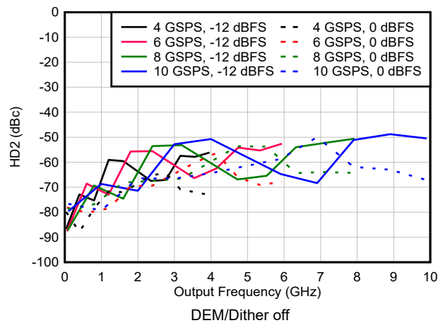
Figure 6-156. HD2 vs Frequency and Sample Rate in DES2X Modes
