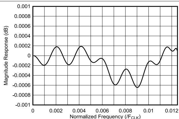
Figure 7-31. 32x Interpolation Filter Passband Response
