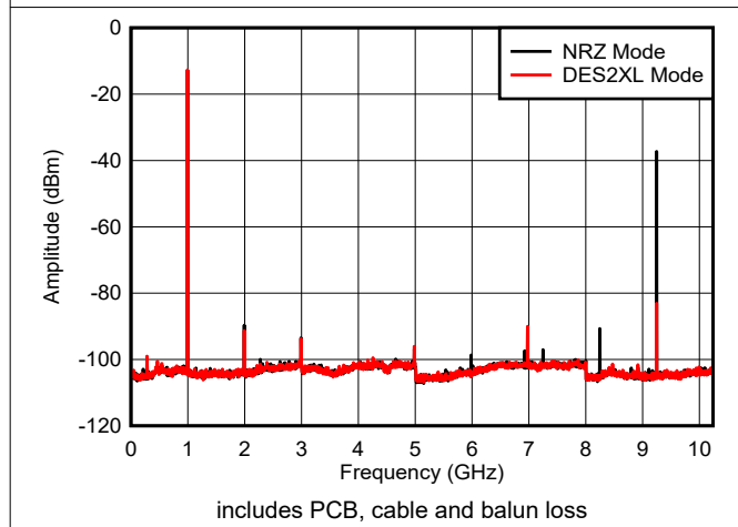
Figure 6-12. f_{\text{OUT}} = 997 \text{ MHz} , -6 dBFS
