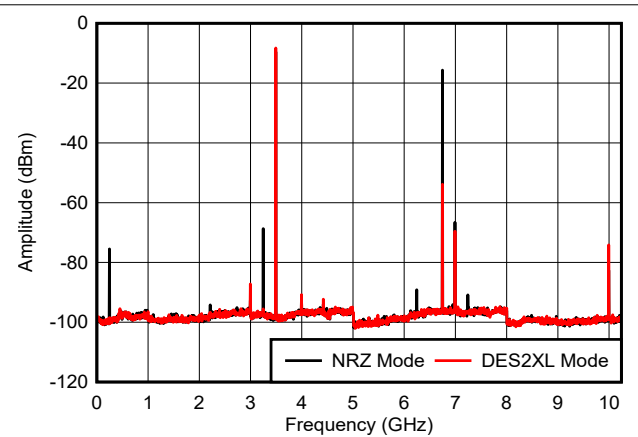
includes PCB, cable and balun loss Figure 6-17. f_{\text{OUT}} = 3497 \text{ MHz} , 0 dBFS
