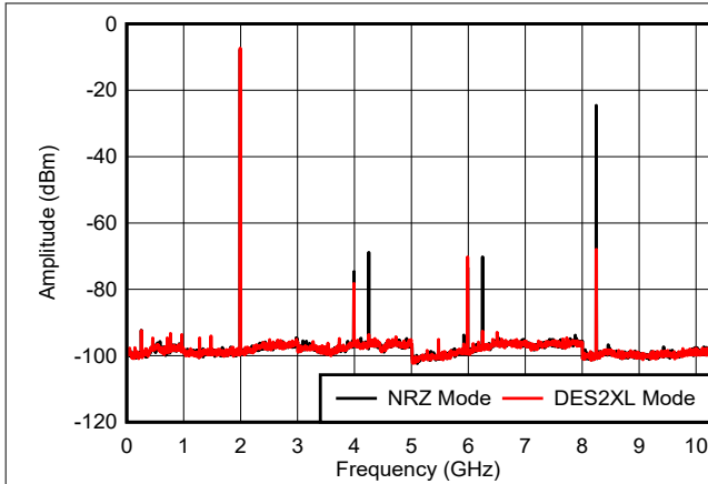
includes PCB, cable and balun loss Figure 6-14. f_{\text{OUT}} = 1997 \text{ MHz} , 0 dBFS
