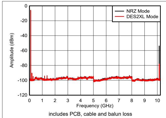
Figure 6-8. f_{\text{OUT}} = 97 \text{ MHz} , 0 dBFS
