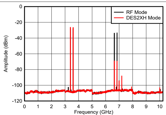
Figure 6-35. Dual Tone, f_{\text{OUT}} = 3497 \text{ MHz} , 0 dBFS
