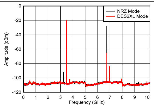
includes PCB, cable and balun loss Figure 6-19. f_{\text{OUT}} = 3497 \text{ MHz} , -12 dBFS
