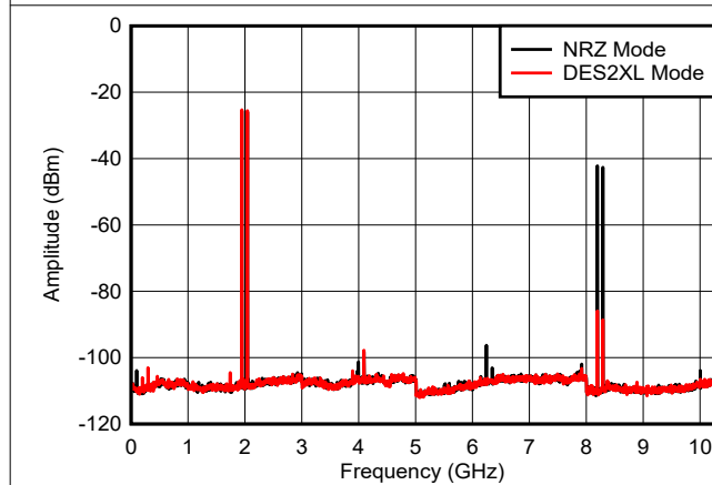
Figure 6-32. Dual Tone, f_{\text{OUT}} = 1997 \text{ MHz} , 0 dBFS
