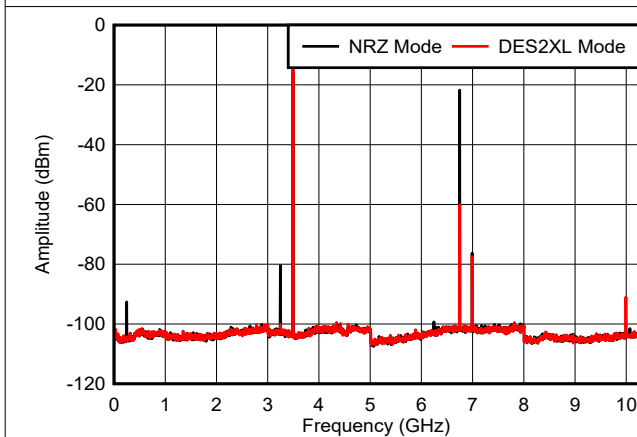
includes PCB, cable and balun loss Figure 6-18. f_{\text{OUT}} = 3497 \text{ MHz} , -6 dBFS
