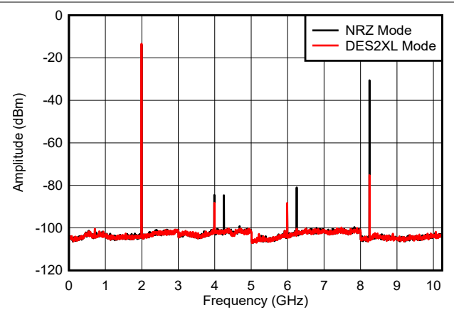
includes PCB, cable and balun loss Figure 6-15. f_{\text{OUT}} = 1997 \text{ MHz} , -6 dBFS
