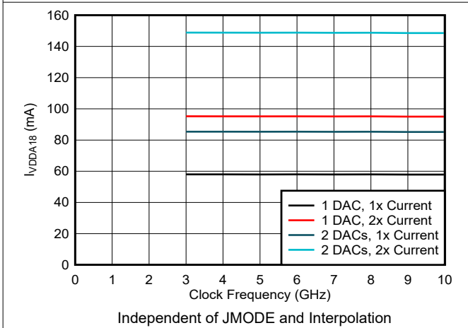
Figure 6-46. VDDA18 Current vs Clock Frequency and DAC Mode
