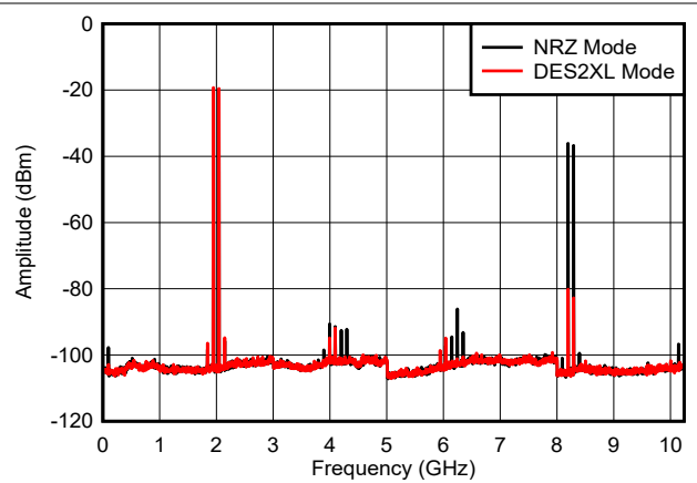
Figure 6-33. Dual Tone, f_{\text{OUT}} = 1997 \text{ MHz} , -6 dBFS
