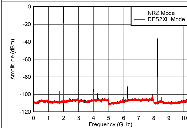
includes PCB, cable and balun loss Figure 6-16. f_{\text{OUT}} = 1997 \text{ MHz} , -12 dBFS
