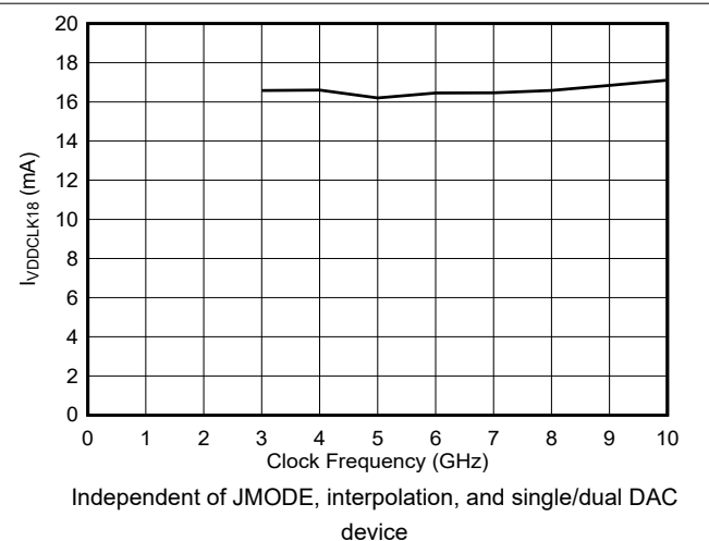
Figure 6-47. VDDCLK18 Current vs Clock Frequency
