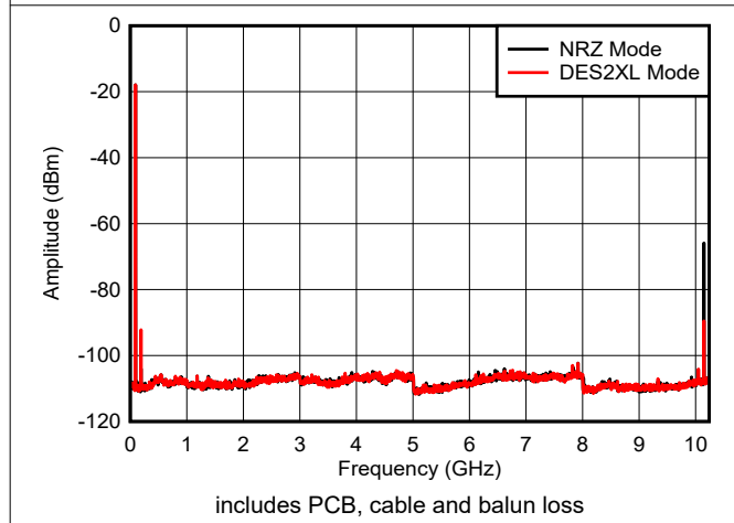
Figure 6-10. f_{\text{OUT}} = 97 \text{ MHz} , -12 dBFS
