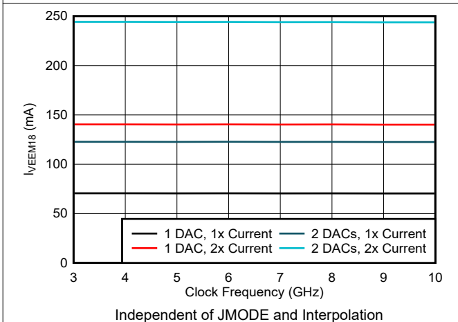
Figure 6-48. VEEM18 Current vs Clock Frequency and Output Current
