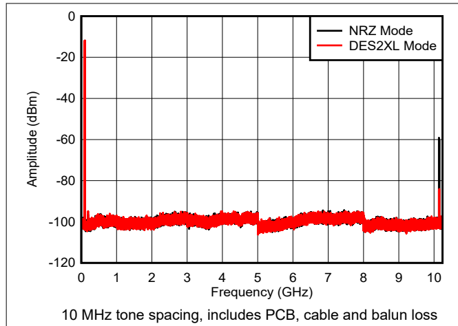
Figure 6-26. Dual Tone, f_{\text{OUT}} = 97\text{ MHz} , 0 dBFS
