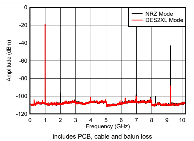
Figure 6-13. f_{\text{OUT}} = 997 \text{ MHz} , -12 dBFS
