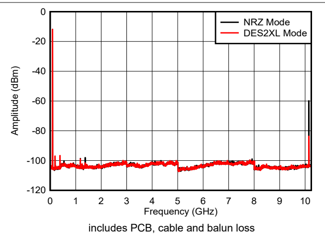
Figure 6-9. f_{\text{OUT}} = 97 \text{ MHz} , -6 dBFS
