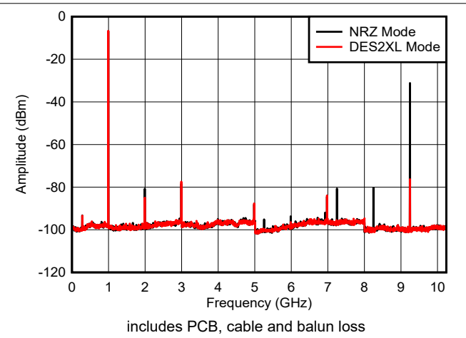
Figure 6-11. f_{\text{OUT}} = 997 \text{ MHz} , 0 dBFS
