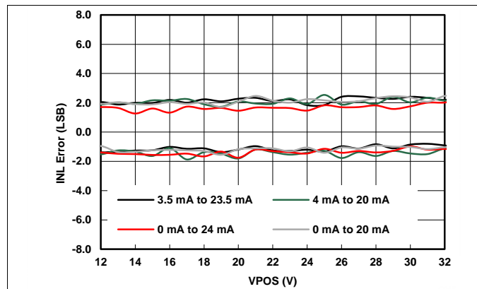
Figure 15. IOU T Linearity Error vs Power Supplies
