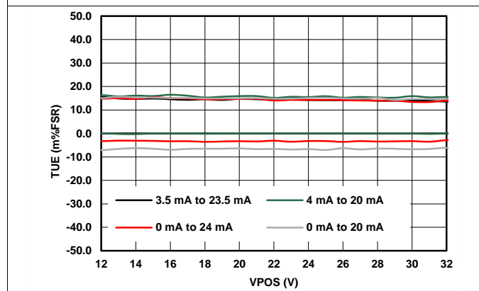
Figure 19. IOU T Total Unadjusted Error vs Power Supplies
