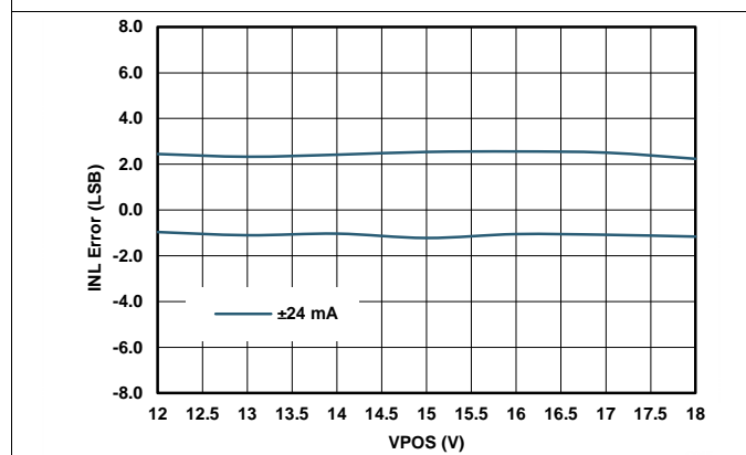
Figure 15. IOU T Linearity Error vs Power Supplies
