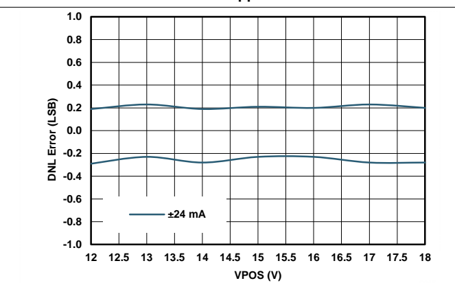
Figure 16. IOU T Differential Linearity Error vs Power Supplies
