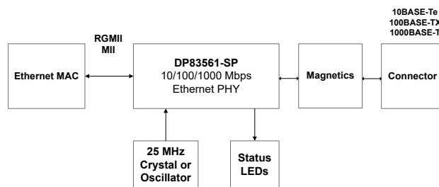
Standard Ethernet System Block Diagram
