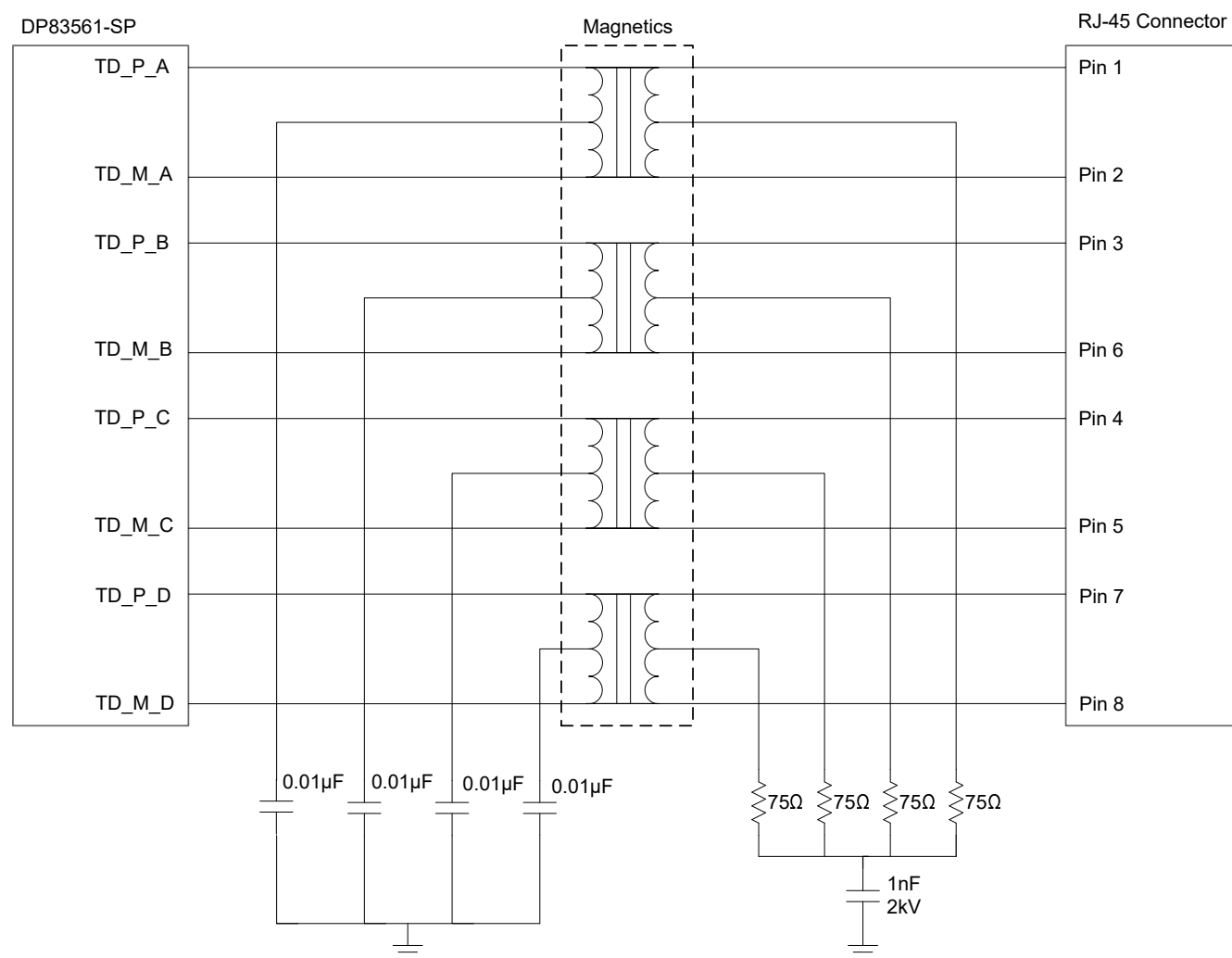
Figure 8-3. Magnetics Connection
