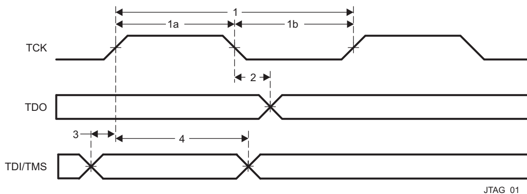
Figure 5-115. JTAG Timing
