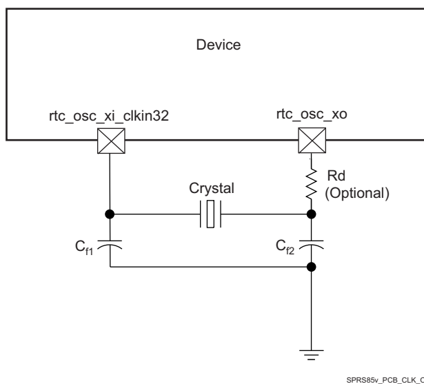
Figure 7-47. Grounding Scheme for Low-Frequency Clock
