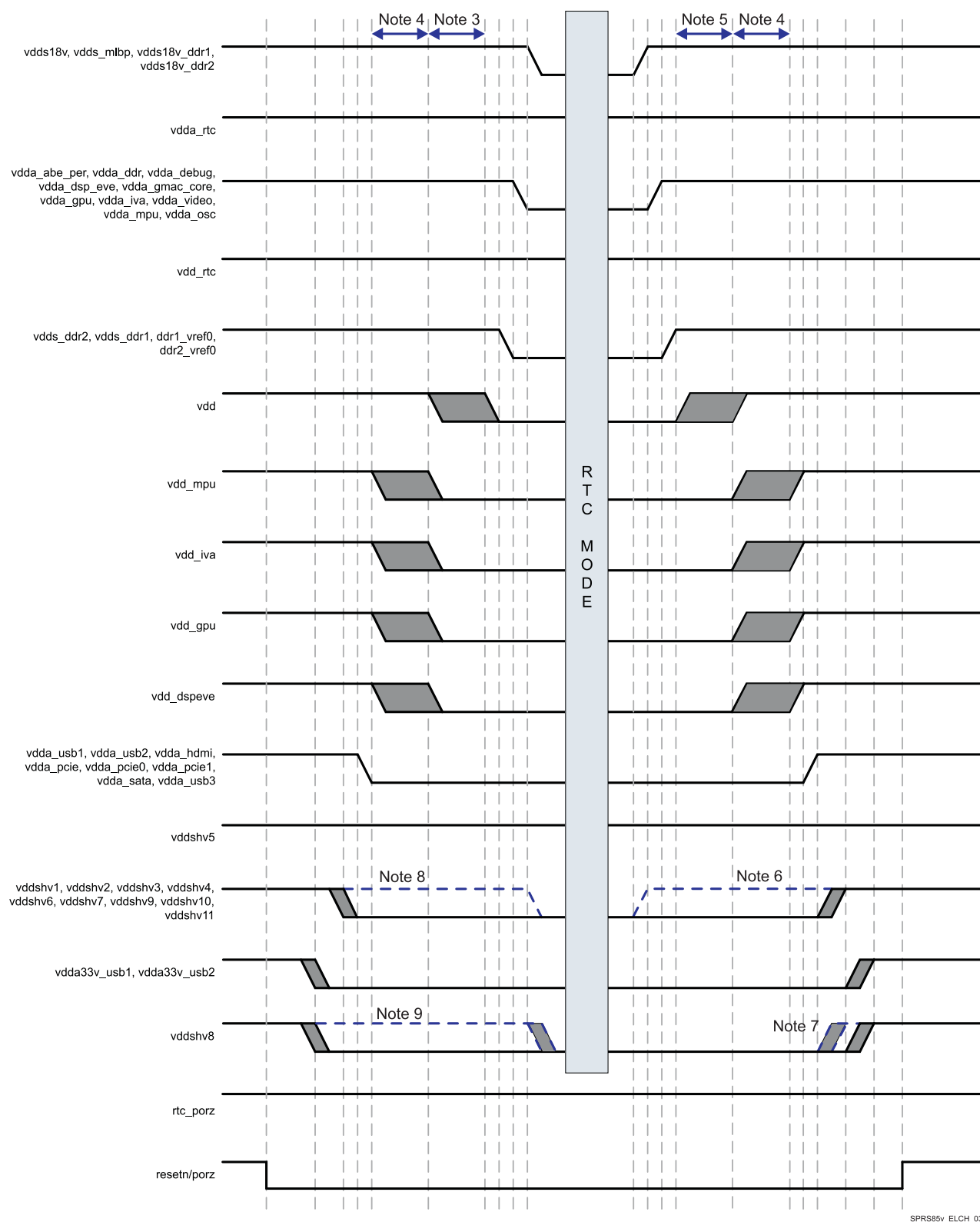
Figure 5-7. RTC Mode Sequencing
