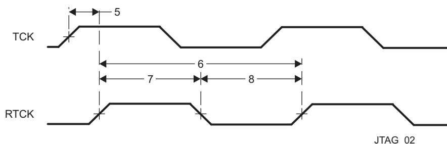
Figure 5-116. JTAG With RTCK Timing
