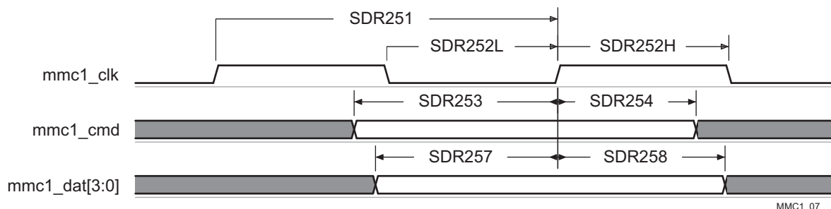
Figure 5-89. MMC/SD/SDIO in - High Speed SDR25 - Receiver Mode
