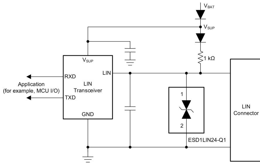
Figure 7-1. Typical Application
