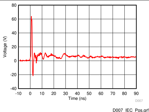
Figure 5-7. +8kV IEC 61000-4-2 Clamping Voltage Waveform, IO Pin to GND
