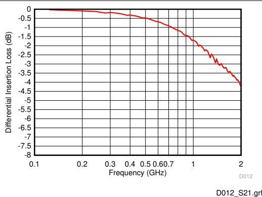
Figure 5-12. Differential Insertion Loss vs. Frequency
