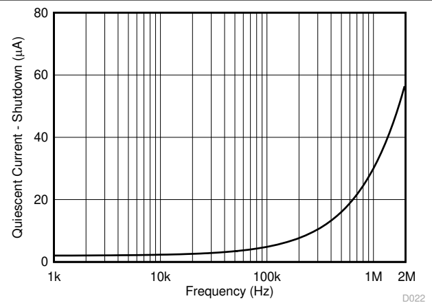
Figure 5-22. Shutdown I_Q vs SCL Frequency
