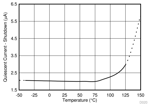
Figure 5-20. Shutdown I_Q vs Temperature
