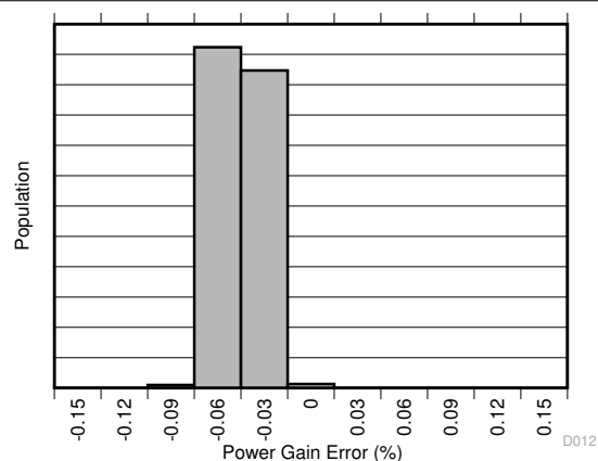
Figure 5-12. Power Gain Error Production Distribution
