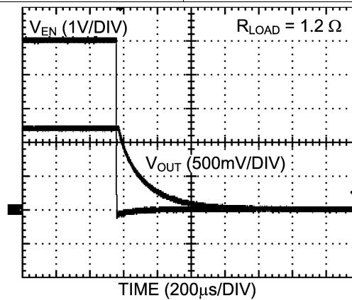
Figure 27. Power Down
