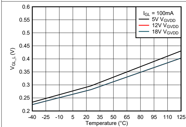
Figure 6-10. GL Output Low Voltage vs Temperature
