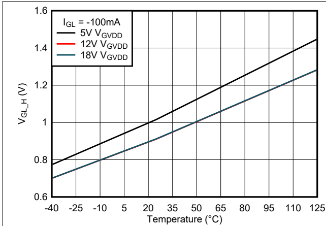
Figure 6-8. GL Output High Voltage vs Temperature
