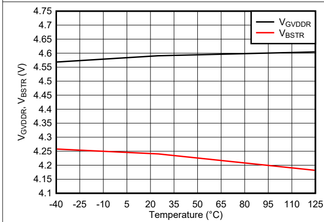
Figure 6-12. GVDD and BST UVLO Thresholds vs Temperature
