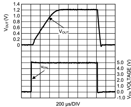
Figure 7-12. Enable - Disable
