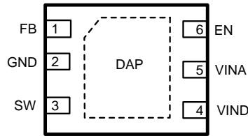
WSON Package 6-Pin Top View
