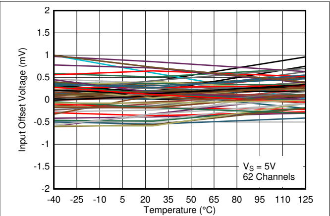
Figure 5-8. Input Offset Voltage vs. Temperature at 5V
