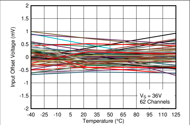
Figure 5-10. Input Offset Voltage vs. Temperature at 36V
