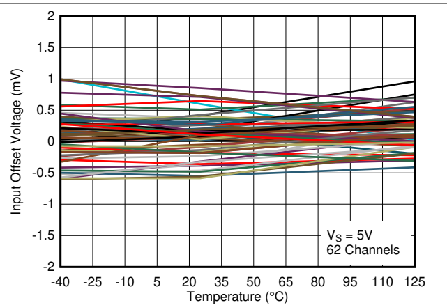
Figure 5-8. Input Offset Voltage vs. Temperature at 5V
