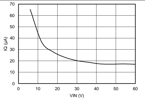
Figure 32. Operating I_Q vs V_{IN} with BIAS Connected to V_{OUT}
