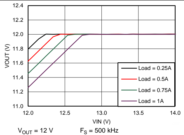
Figure 74. Dropout Curve
