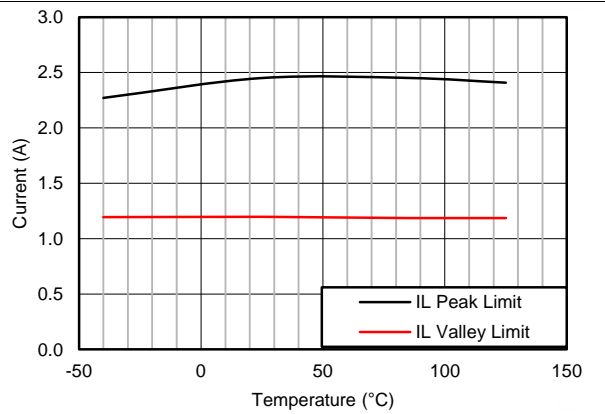
Figure 31. Peak and Valley Current Limits vs Junction Temperature
