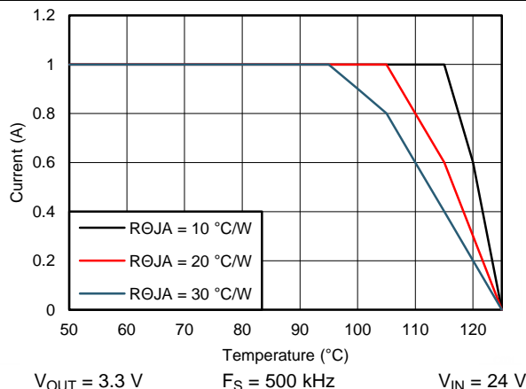
Figure 52. Derating Curve
