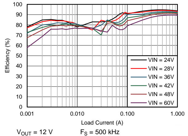
Figure 72. Efficiency
