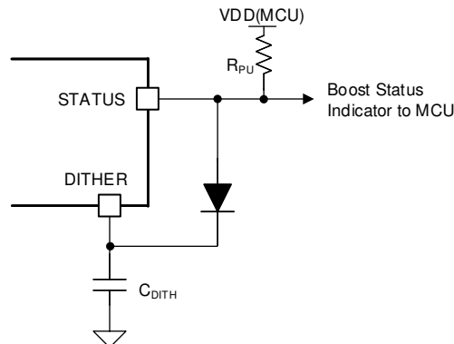
Figure 9-12. Enable Clock Dithering and Internal Charge Pump Together
