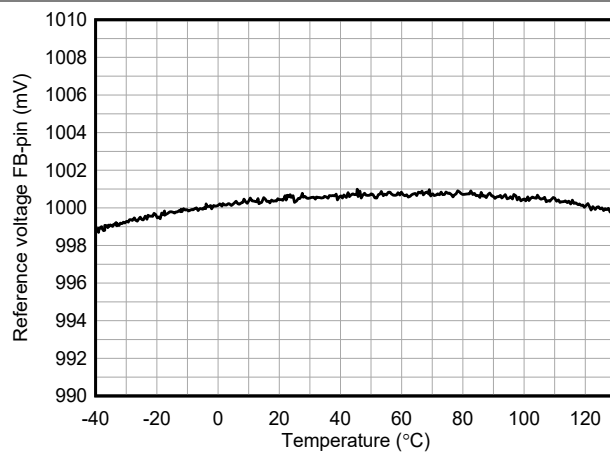
Figure 6-7. FB Pin Reference Voltage vs Temperature
