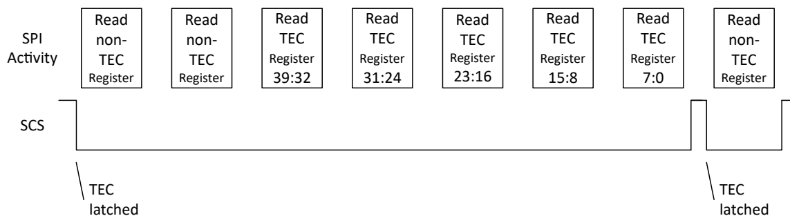
Figure 8-34. TEC Multibyte Read
