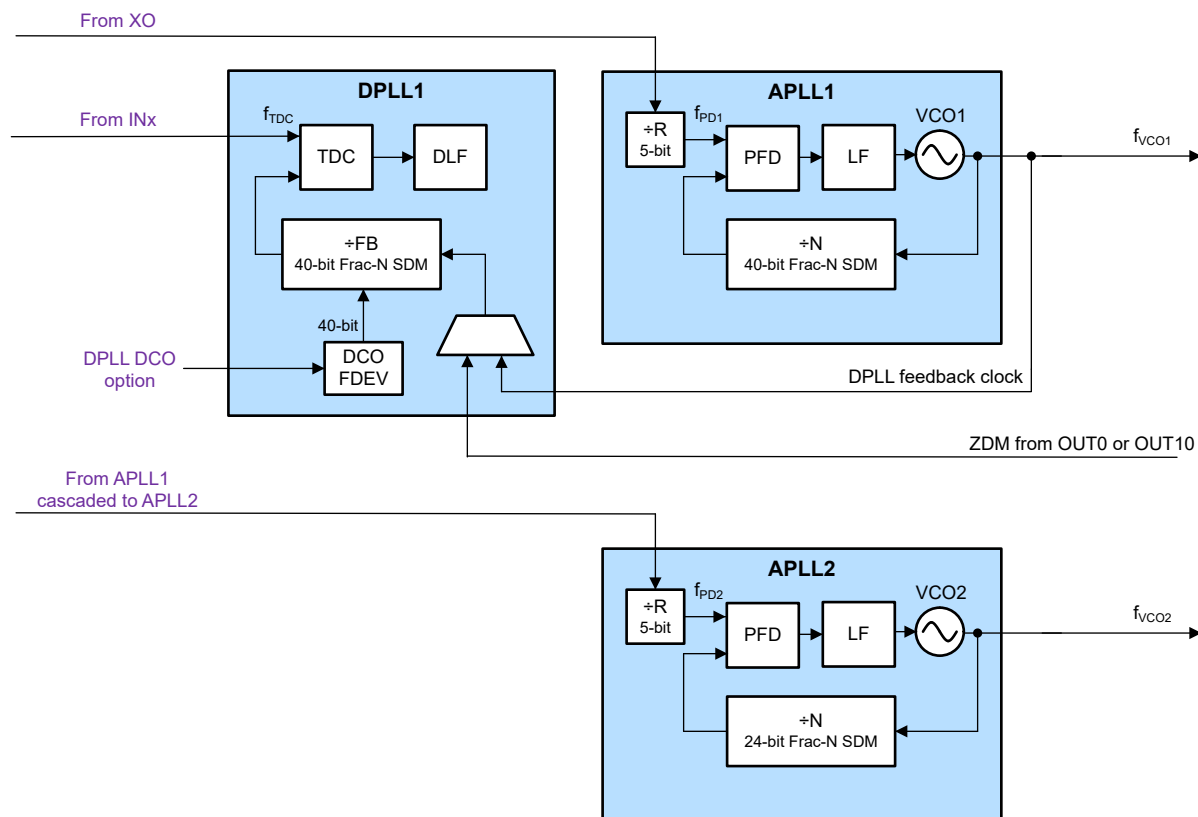
Figure 8-4. APPL Cascaded With DPLL Example
