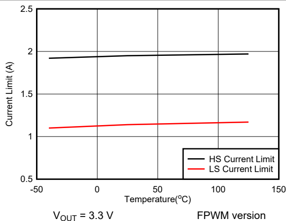
Figure 6-5. High-Side and Low-Side Current Limit vs Temperature
