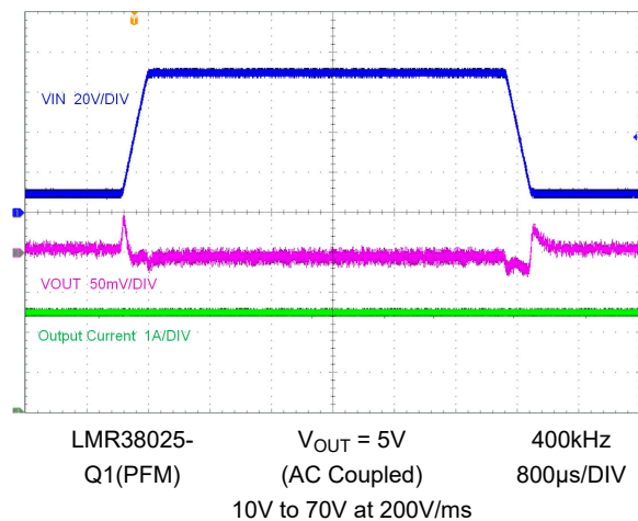
Figure 8-12. Line Transient
