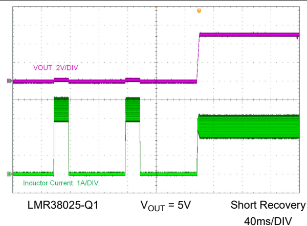
Figure 8-8. Short-Circuit Recovery
