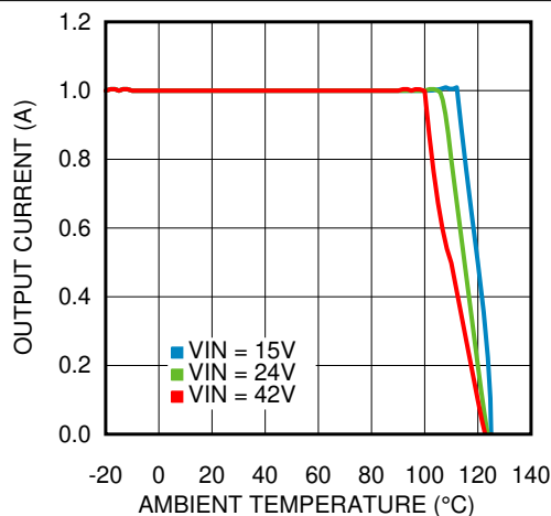
Figure 6-26. Thermal Derating V_{OUT} = 12\text{ V} , R_{\theta JA} = 20^\circ\text{C/W}
