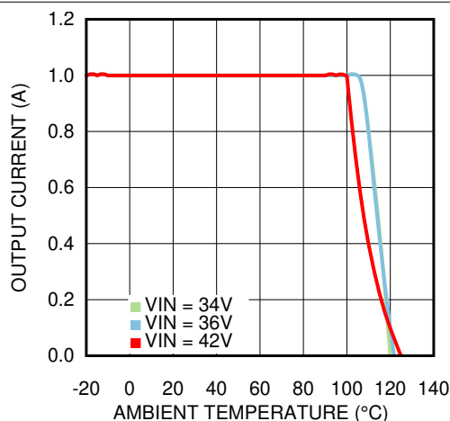
Figure 6-30. Thermal Derating V_{OUT} = 30\text{ V} , R_{\theta JA} = 20^\circ\text{C/W}
