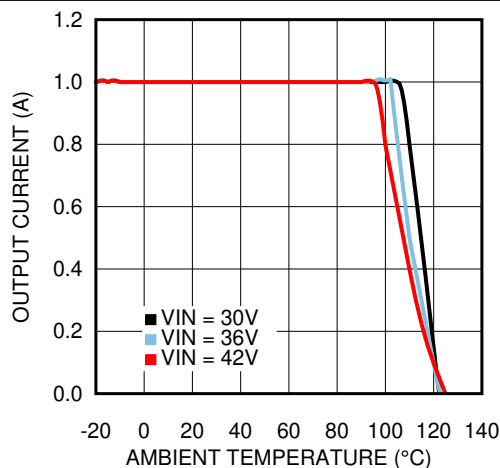
Figure 6-28. Thermal Derating V_{OUT} = 24\text{ V} , R_{\theta JA} = 20^\circ\text{C/W}
