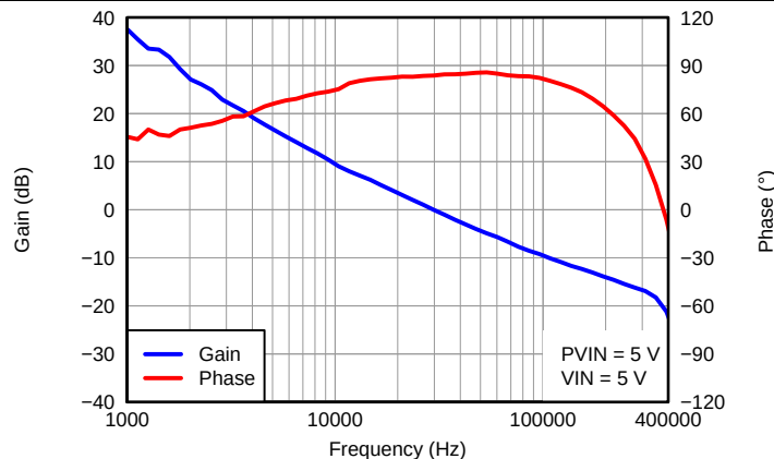
Figure 10. VOUT=1.2 V, IOUT=3 A, COUT1=47 µF ceramic, COUT2= 330 µF POSCAP, fSW=480 kHz
