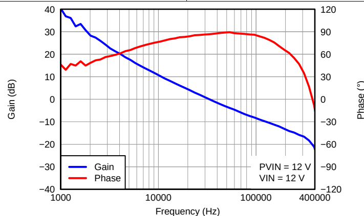
Figure 5. V OUT =1.2 V, I OUT =3 A, C OUT1 =47 µF ceramic, C OUT2 = 330 µF POSCAP, f SW =480 kHz
