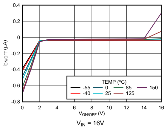
Figure 5-39. ON/OFF Pin Current vs V_{ON/OFF} (New Chip)
