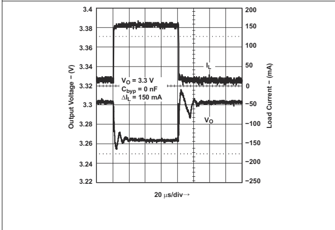
Figure 7-7. Load Transient Response for Legacy Chip
