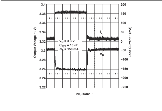
Figure 7-5. Load Transient Response for Legacy Chip
