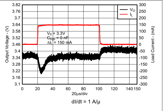
Figure 7-8. Load Transient Response for New Chip
