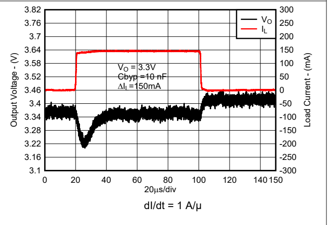
Figure 7-6. Load Transient for New Chip
