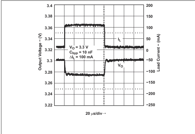
Figure 7-3. Load Transient Response for Legacy Chip
