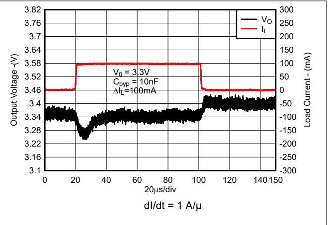
Figure 7-4. Load Transient Response for New Chip
