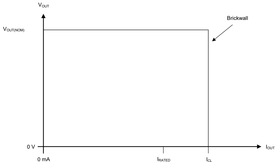
Figure 6-3. Current Limit
