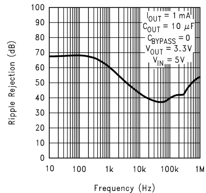
Figure 5-6. Ripple Rejection vs Frequency (Legacy Chip)
