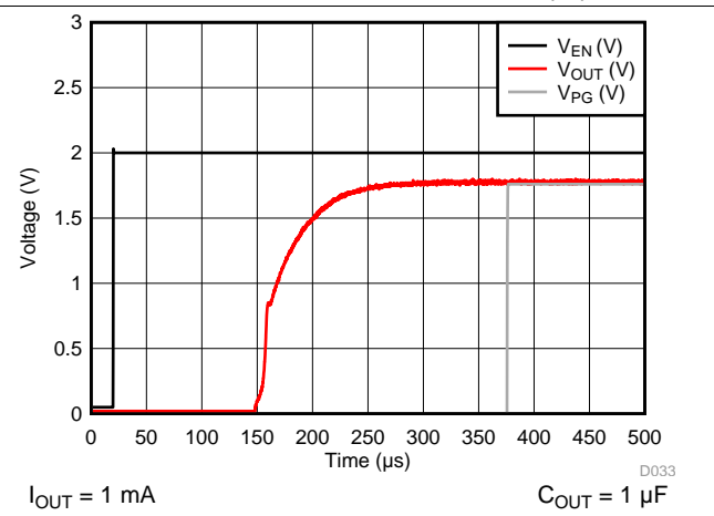
Figure 40. LP5912-1.8 V_{OUT} vs V_{EN(ON)}
