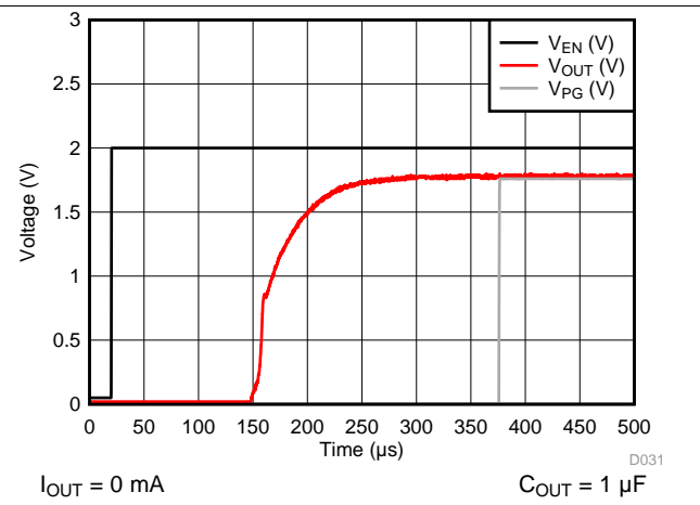
Figure 38. LP5912-1.8 V_{OUT} vs V_{EN(ON)}
