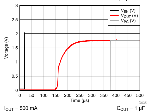
Figure 42. LP5912-1.8 V_{OUT} vs V_{EN(ON)}
