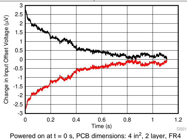
Figure 53. Warm-Up Time
