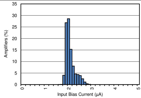
Figure 38. Input Bias Current Distribution
