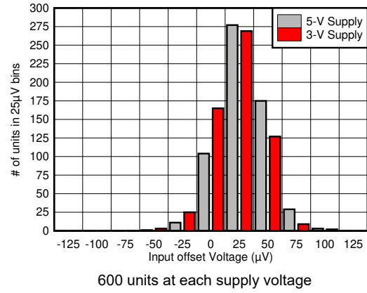
Figure 6-44. Input Offset Voltage Distribution
