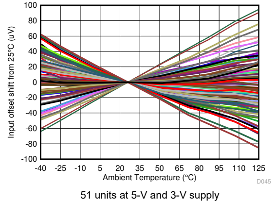
Figure 6-46. Input Offset Voltage vs Temperature
