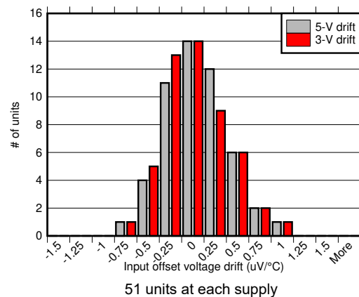
Figure 6-48. Input Offset Voltage Drift Distribution
