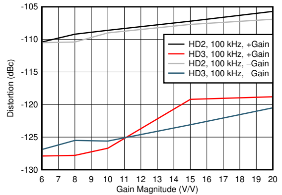
See Figure 8-1, Figure 8-2, Table 8-1, and Table 8-2 2-k \Omega load, 2 V_{PP}
