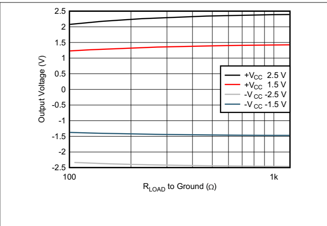
Figure 6-56. Output Voltage Swing vs Load Resistor
