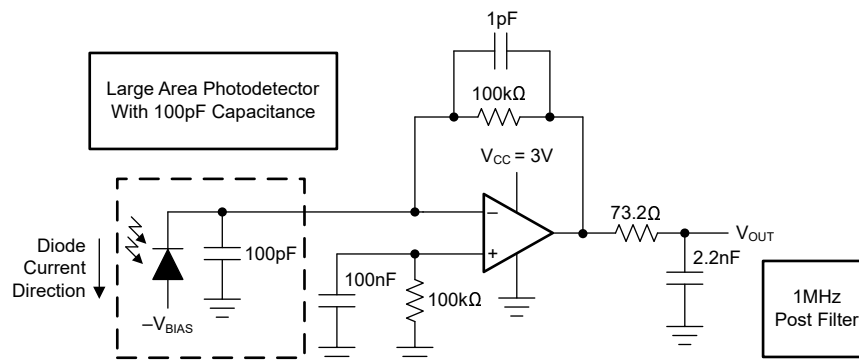
Single 3V Supply, < 3mW Photodiode Amplifier With < 1.1pA/√Hz Total Input-Referred Current Noise and 100kΩ Gain With Overall 1MHz SSBW
