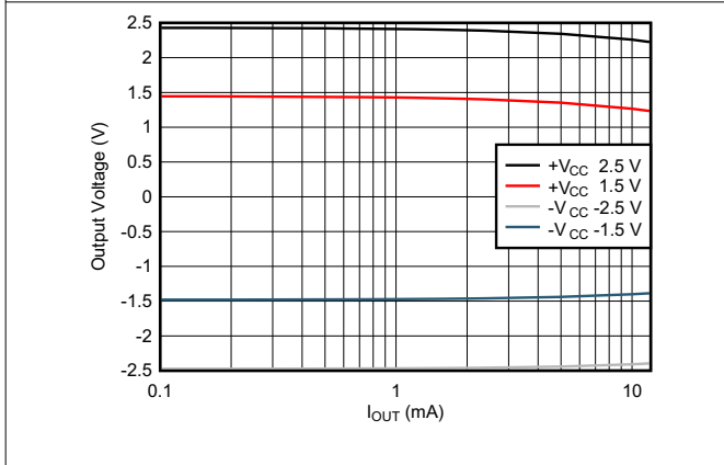
Figure 6-57. Output Saturation Voltage vs Load Current
