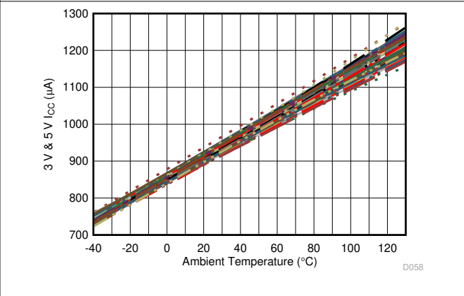
Figure 6-58. Quiescent Current vs Temperature
