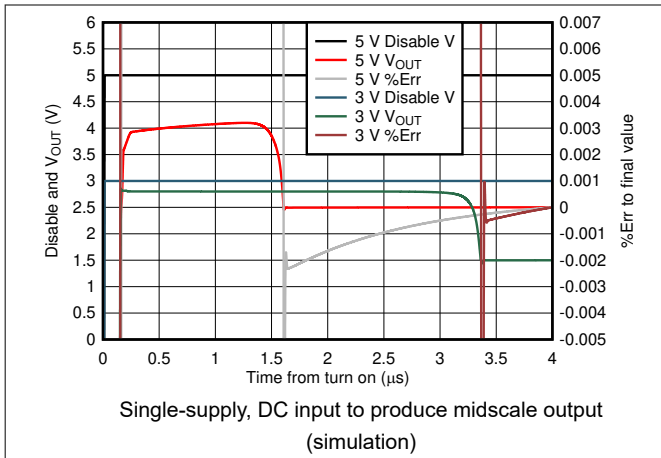
Figure 6-55. Gain of 10-V/V Turn-On Time to Final DC Value at Midscale
