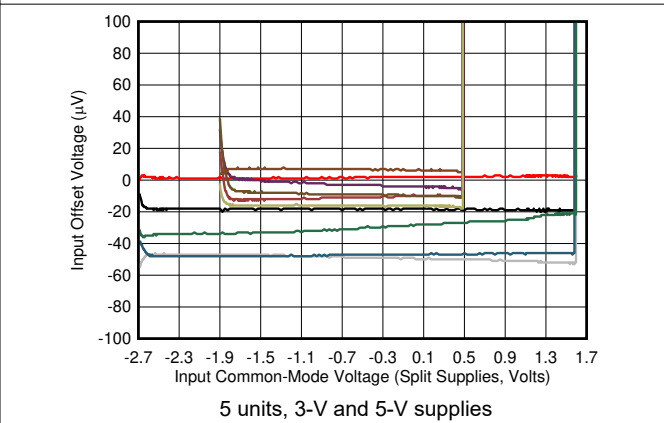
Figure 6-60. Input Offset Voltage vs Input Common-Mode Voltage
