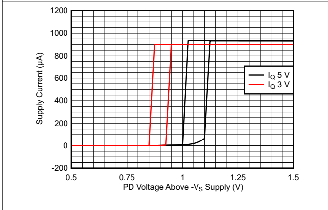
Figure 6-59. Supply Current vs Power-Down Voltage: Turn On Higher Than Turn Off
