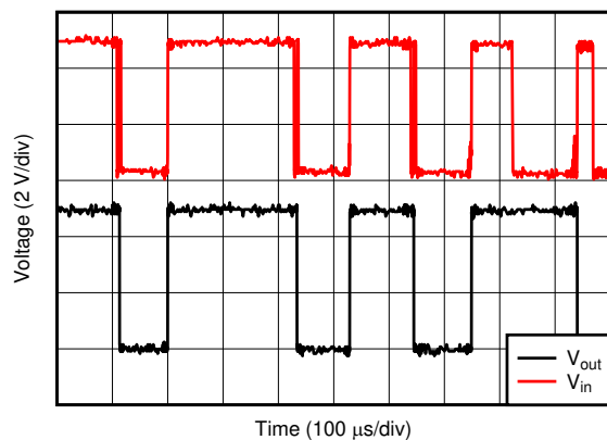
Figure 8-2. Circuit Response Without RC Debounce V_{in} := \text{CLK Input}, V_{out} := \text{Q Output}
