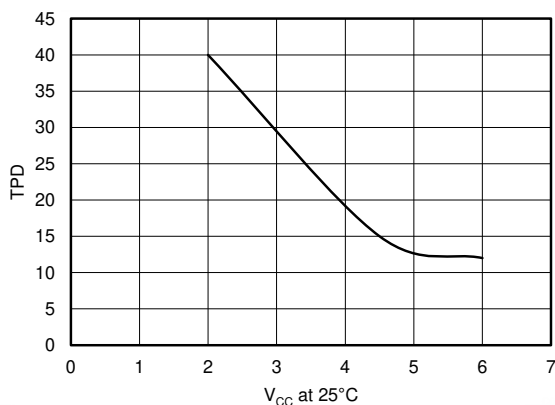
Figure 5-1. TPD vs V_{CC} at 25^\circ\text{C}
