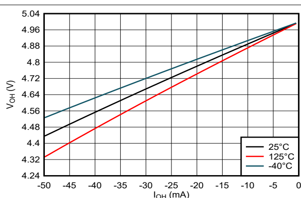
Figure 5-2. Output Voltage vs Current in HIGH State; 5V Supply
