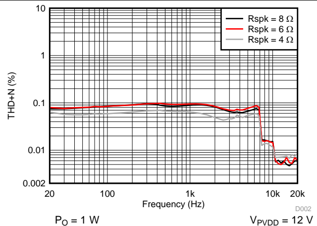
Figure 19. THD+N vs Frequency – PBTL
