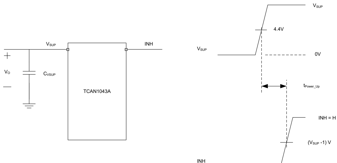
Figure 6-10. Power-Up Timing
