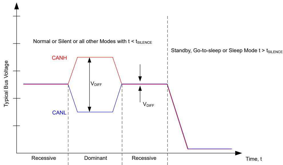
Figure 7-11. Bus States
