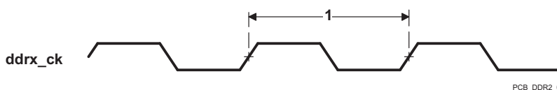
Figure 7-49. DDR2 Memory Controller Clock Timing
