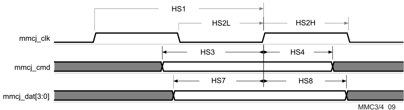
Figure 5-98. MMC/SD/SDIOj in - High Speed - Receiver Mode
