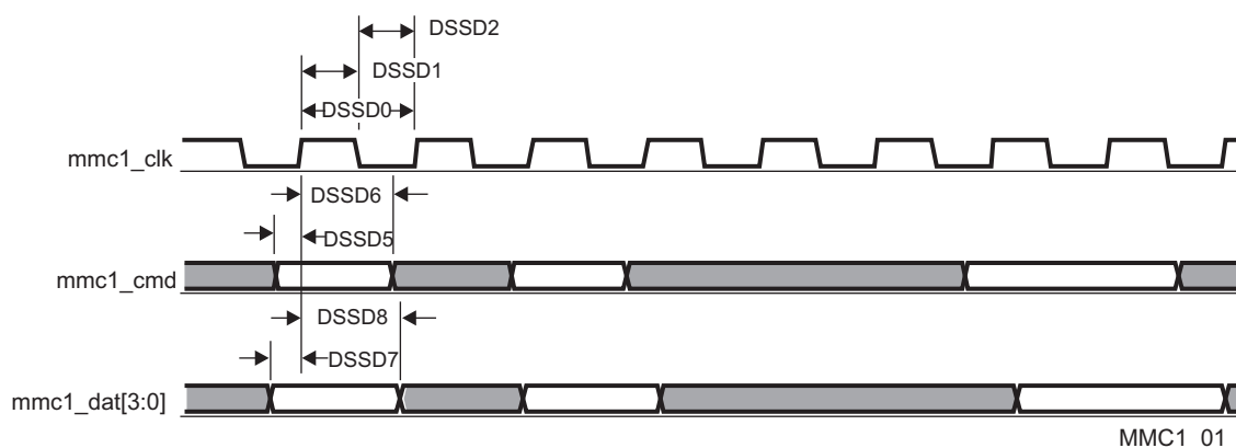
Figure 5-75. MMC/SD/SDIO in - Default Speed - Receiver Mode
