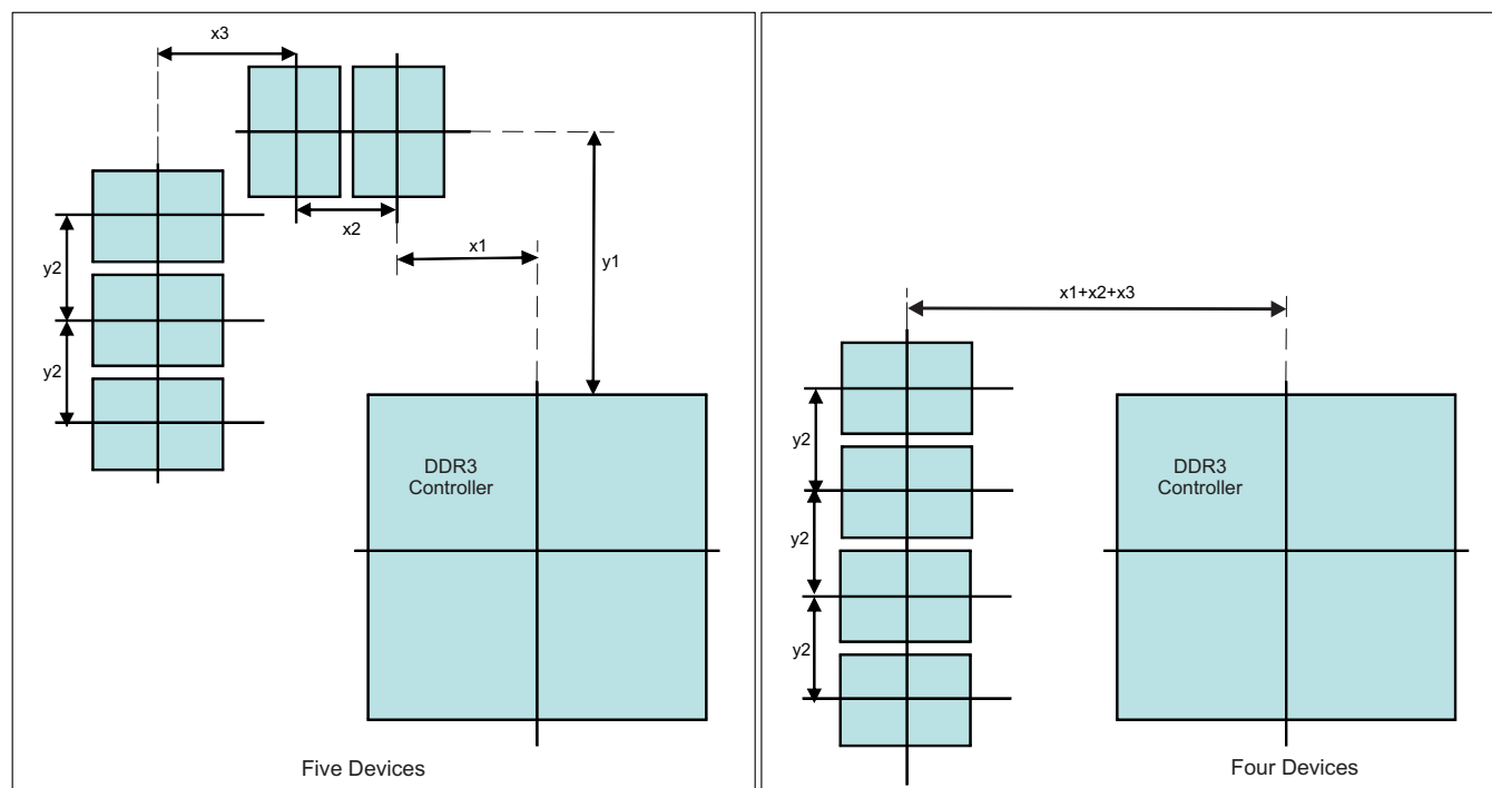
Figure 7-60. Placement Specifications
