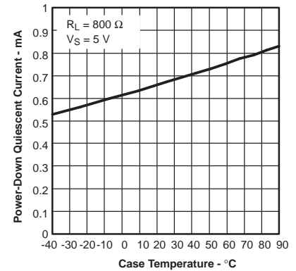
POWER-DOWN QUIESCIENT CURRENT vs CASE TEMPERATURE
