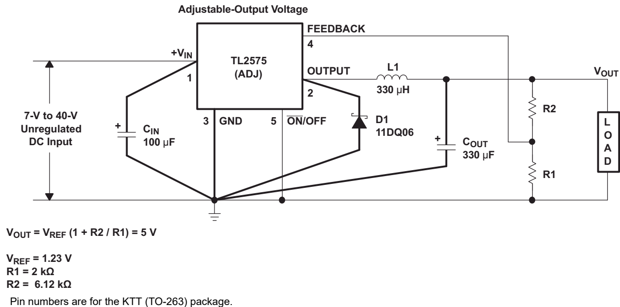
Figure 7-1. Test Circuits and Layout Guidelines
