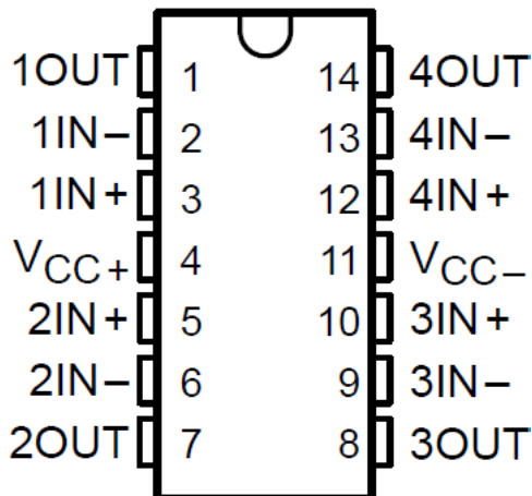
Figure 4-3. TLE2064, TLE2064A, and TLE2064B D, J, N, or W Package (Top View)
