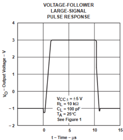
Figure 5-9. Voltage Follower Large Signal Pulse Response
