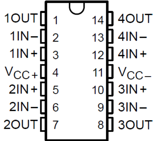
Figure 4-4. TLE2064, TLE2064A, and TLE2064B D, J, N, or W Package (Top View)
