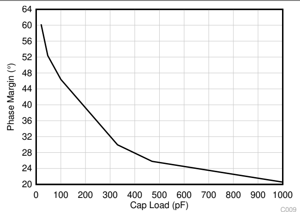
Figure 5-18. Phase Margin vs Capacitive Load
