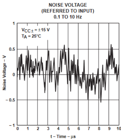
Figure 5-11. Noise Voltage
