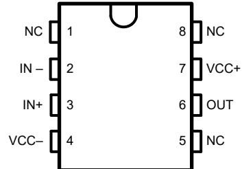
Figure 4-2. TLE2061, TLE2061A,D, P Package (Top View)
