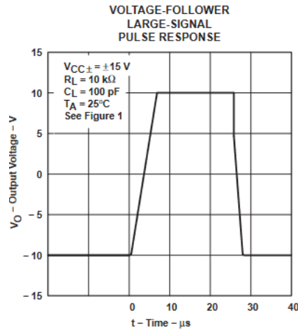
Figure 5-10. Voltage Follower Large Signal Pulse Response
